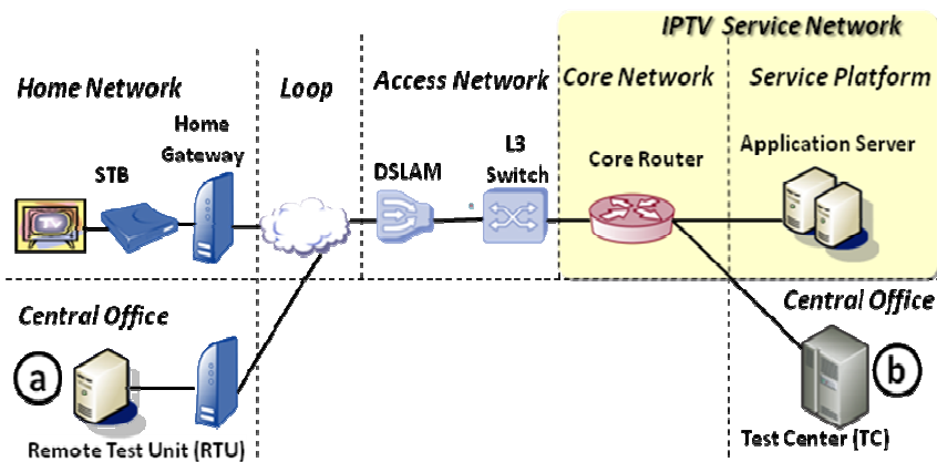
Figure 9. The RTU and TC configuration
