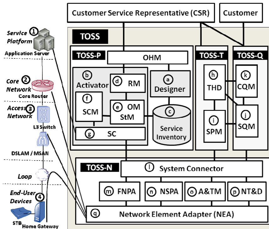
Figure 2. TOSS architecture (and an example of management for IPTV)
