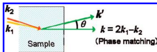
FIGURE 3. Phase matching condition and spatial distribution of CARS signal.
