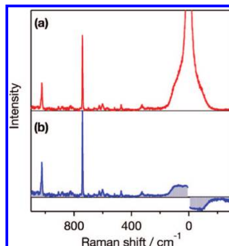
FIGURE 1. The observed (a) and reduced (b) Raman spectra of C_4 -mim[PF 6 ].
