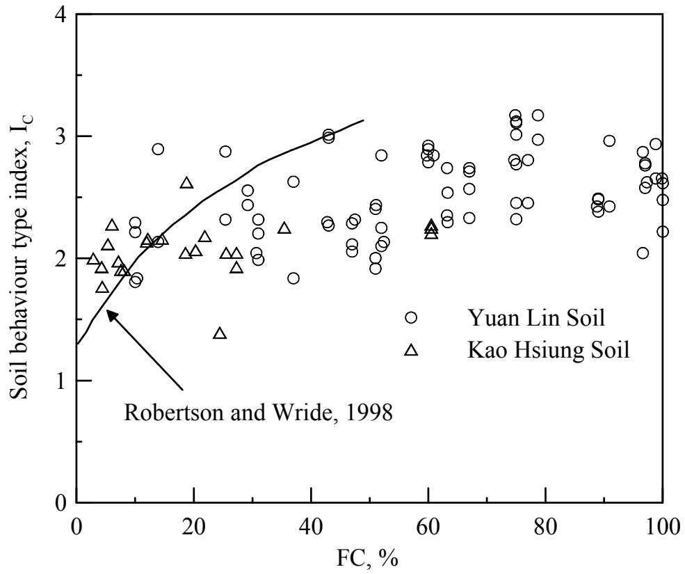
Figure 1. I_C versus fines contents.
