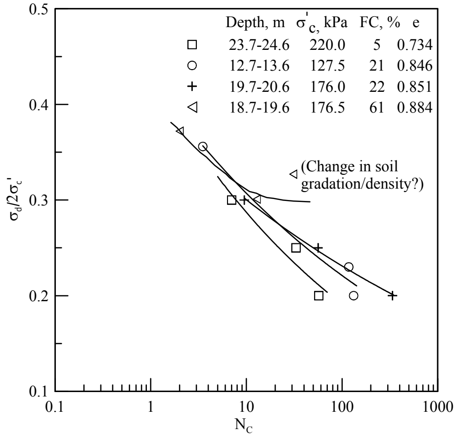
Figure 7. Cyclic triaxial test results of KHS specimens recovered by the gel-push sampler.
