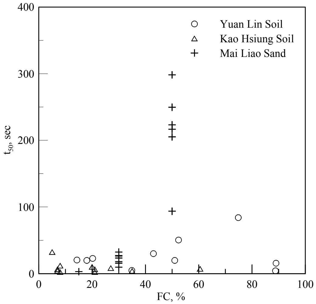
Figure 12. t_{50} versus fines contents
