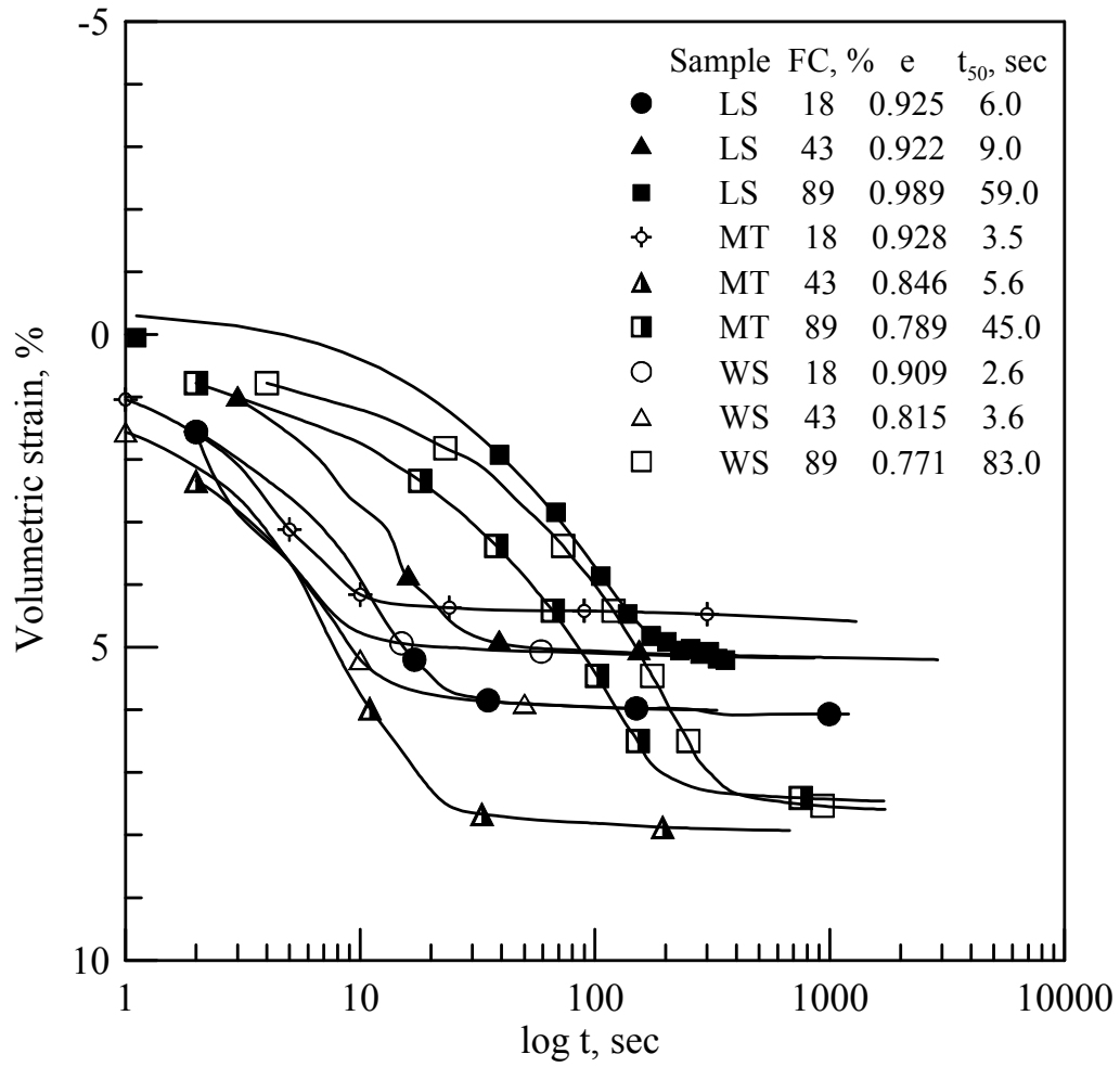
Figure 6. Pore pressure dissipation following a cyclic triaxial test.
