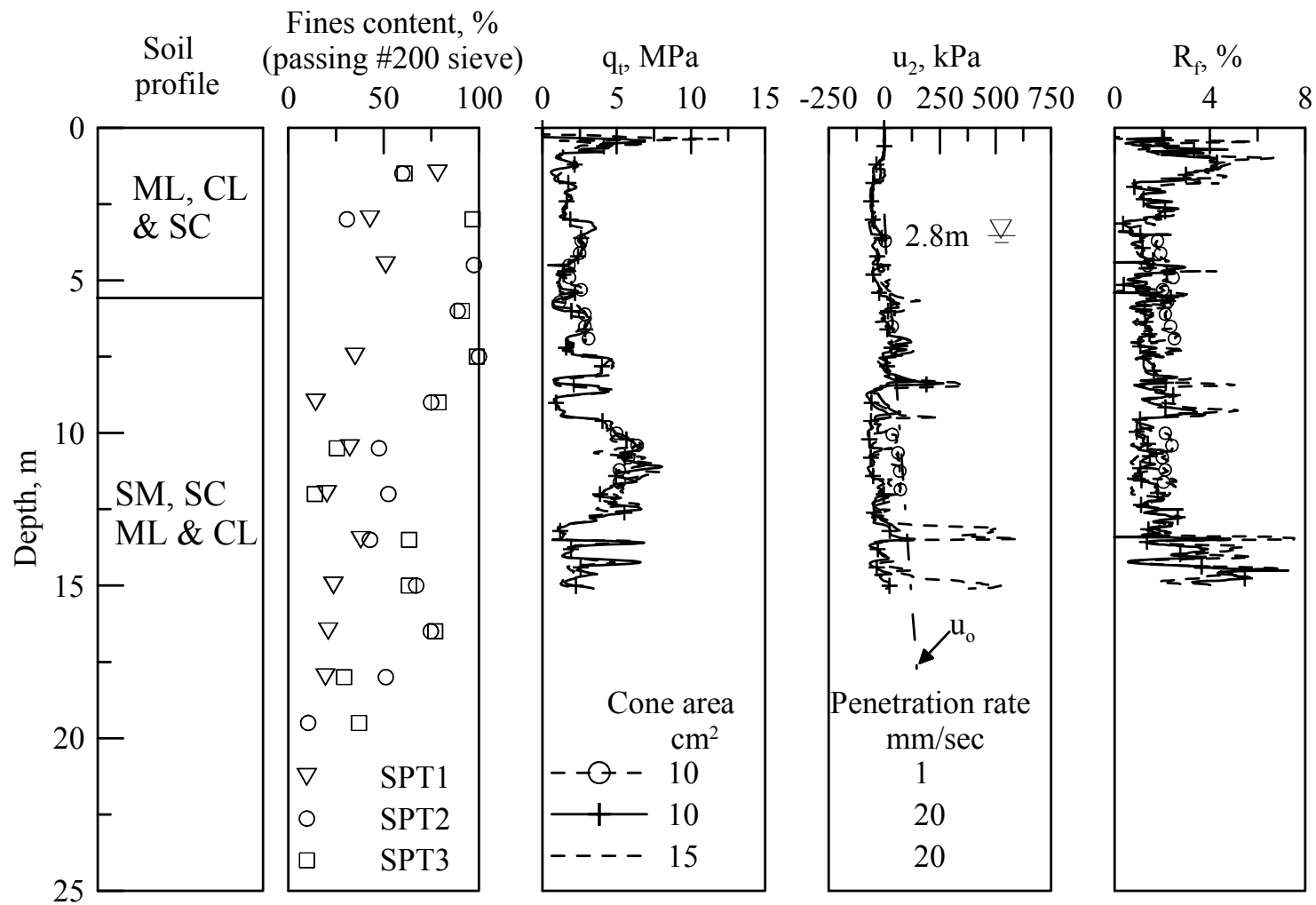
Figure 8. CPTU profiles at Yuan Lin test site.
