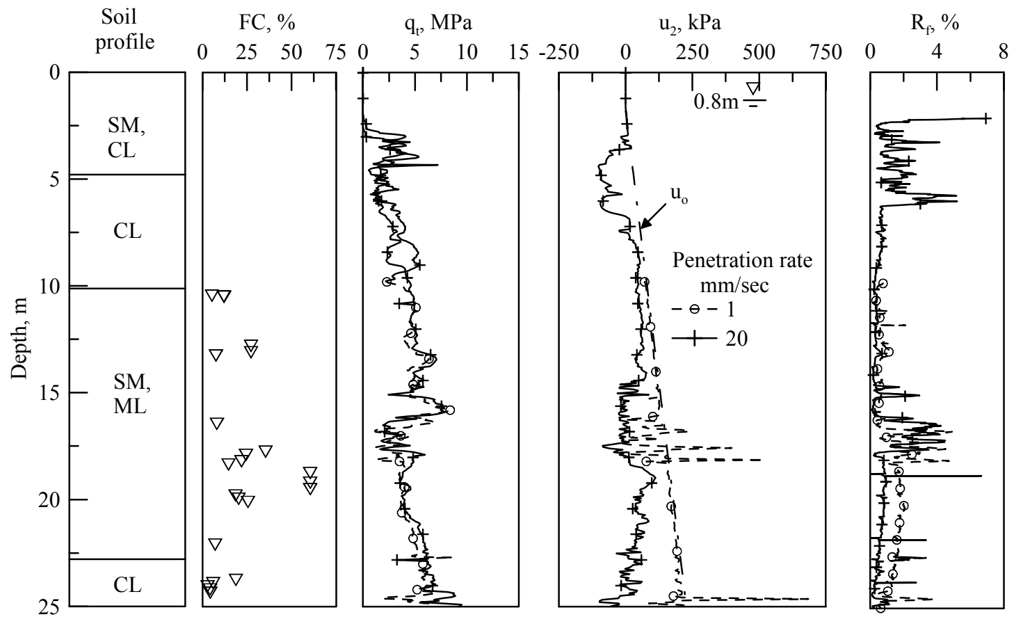
Figure 9. CPTU profiles at Kao Hsiung test site.
