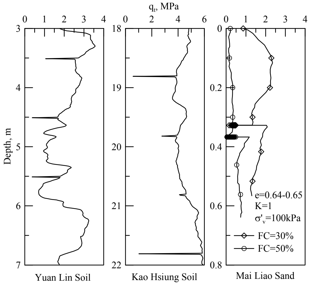
Figure 10. q_t profiles with CPT dissipation tests.
