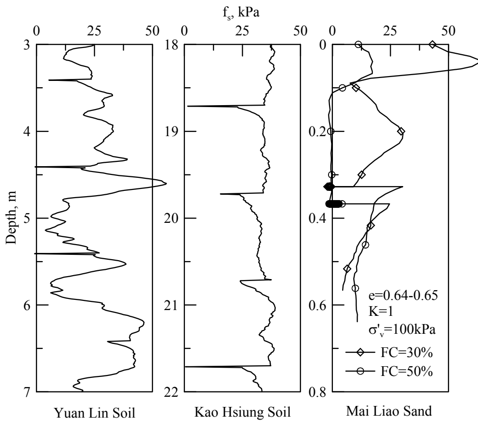
Figure 11. f_s profiles with CPT dissipation tests.
