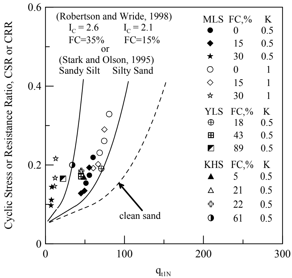
Figure 14. Correlation between CRR and q_{t1N} .
