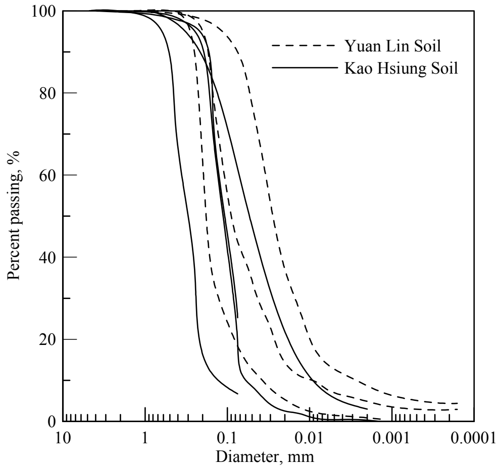
Figure 3. Grain size distribution curves of MLS and YLS.
