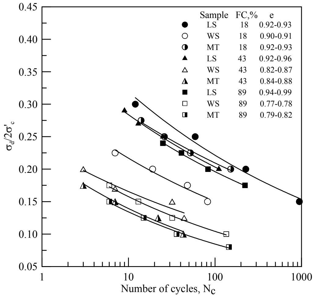
Figure 5. Cyclic triaxial test results of YLS specimens.
