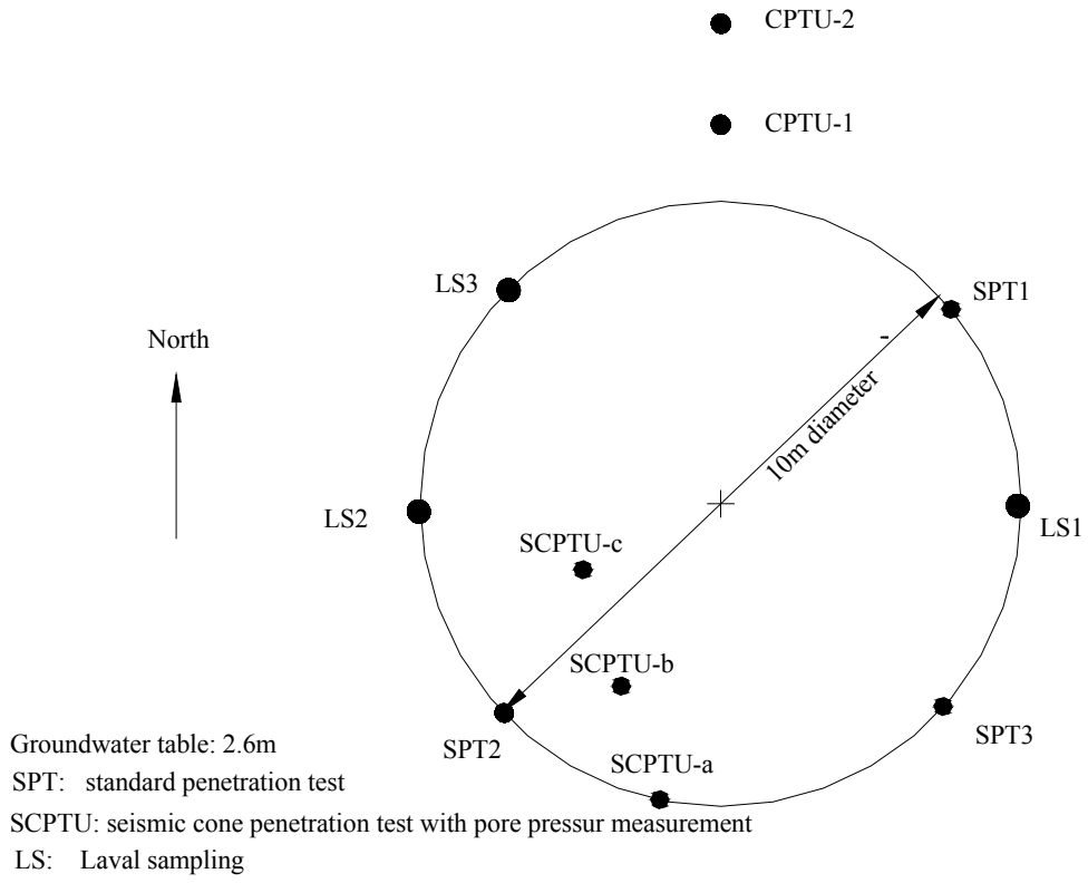
Figure 4. Field test and sampling locations at Yuan Lin test site.
