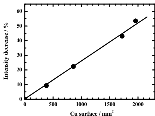
Figure 3-7. For poly(3-octylpyrrole)squaraine in trichloromethane solution, the decrease of absorbance at 543.6 nm in 1 h vs. area of copper surface at 295 K.
