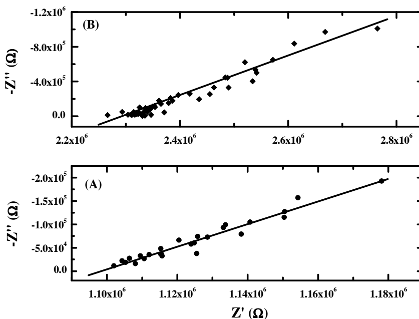
Figure 2-20. Impedance plots of poly(3-octylpyrrole)squaraine (3.5 mg/L) in solution: (A) the linear conformer and (B) the folded conformer.
