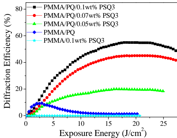
Figure 4. Holographic diffraction efficiencies of the photopolymers.
