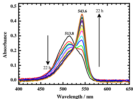
Figure 2-9. Temporal variation of absorption spectra of poly(3-octylpyrrole)squaraine in trichloromethane at 323 K after removal of the copper plate following its insertion for 11 h: scans were made at hourly intervals from 0 to 12 h, then at 15, 19 and 22 h.
