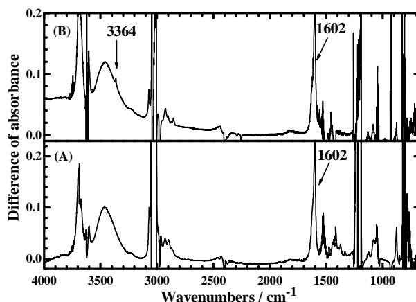
Figure 2-13. Difference IR absorption spectra in trichloromethane solution with optical path 1 mm relative to pure solvent: (A) poly(3-octylpyrrole)squaraine in trichloromethane solution, (B) the same solution into which a Cu plate is inserted.
