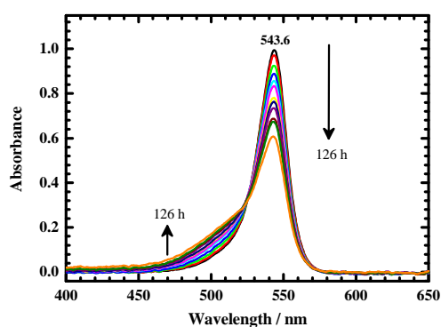
Figure 2-16. Temporal variation of visible absorption spectra of poly(3-octylpyrrole)squaraine in trichloromethane in a quartz cell to which was added a saturated solution of Ca^{2+} in trichloromethane: before addition (black curve), and after 0.5, 1, 2, 3, 7, 10, 19, 33, 46, 126 (blue curve) h. For this reaction we prepared a saturated solution of Ca^{2+} in trichloromethane over Ca(ClO_4)_2 \cdot 4H_2O .
