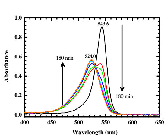
Figure 2-15. Temporal variation of visible absorption spectra of poly(3-octylpyrrole)squaraine in trichloromethane (3 mL) in a quartz cell (length 1 cm of optical path) to which was added a saturated solution (10 \mu\text{L} ) of \text{Cu}^{2+} in trichloromethane: before addition (black curve), and after 2, 5, 10, 30, 60, 120, 180 (orange curve) min. For this reaction we prepared a saturated solution of \text{Cu}^{2+} in trichloromethane over \text{Cu}(\text{ClO}_4)_2 \cdot 6\text{H}_2\text{O} .
