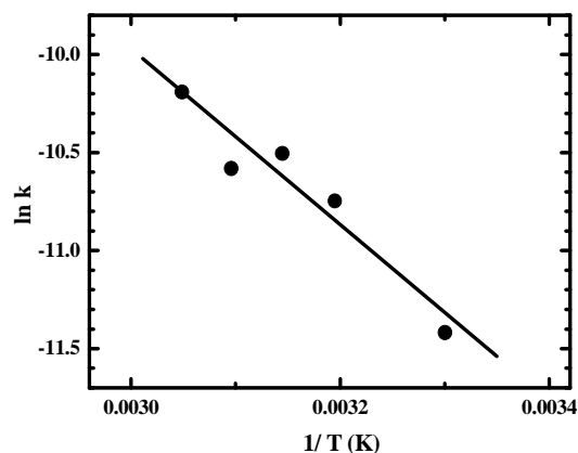
Figure 2-10. Absorbance decrease at 513.8 nm in 1 h vs. temperature after removal of inserted copper plates from P3 solutions.
