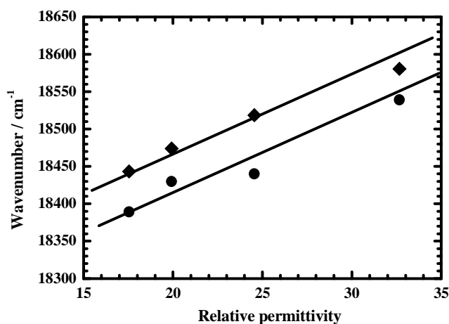
Figure 1-7. Wavenumber of absorption maxima of P1 (solid circle) and P3 (solid diamond), as synthesized, versus relative permittivity of methanol, ethanol, isopropanol and 1-butanol.
