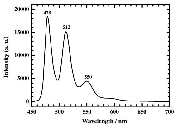
Figure 2-19. Photoluminescent spectrum of 2,3-benzanthracene under the same optical conditions; the spectrum was used as an external standard.
