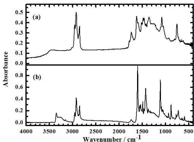
Figure 1-1. IR absorption spectra of polysquaraines as synthesized, in the spectral range 400–4000 \text{cm}^{-1} : (a) P1 ; (b) P3 .
