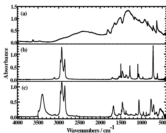
Figure 1-2. IR absorption spectra of monomers in the spectral range 400–4000 \text{cm}^{-1} (a) squaric acid; (b) 1-octylpyrrole; and (c) 3-octylpyrrole.
