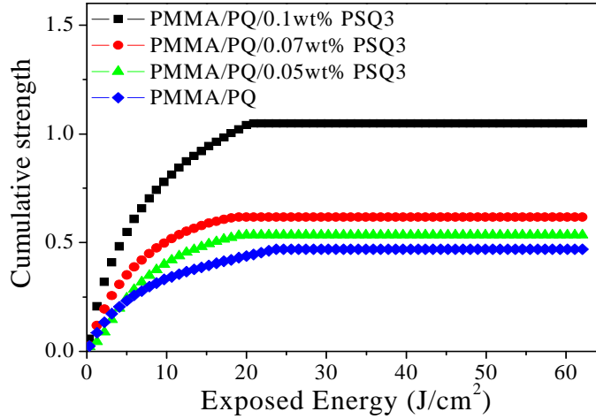
Figure 5. Running curves for multiple-hologram recording in the photopolymers.
