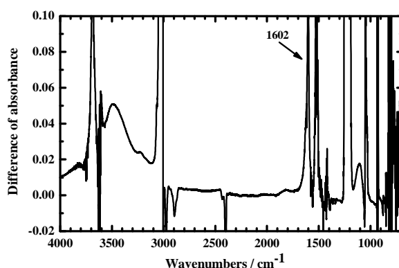
Figure 2-17. Difference IR absorption spectrum of poly(3-octylpyrrole)squaraine in trichloromethane to which was added Cu^{2+} in solution.
