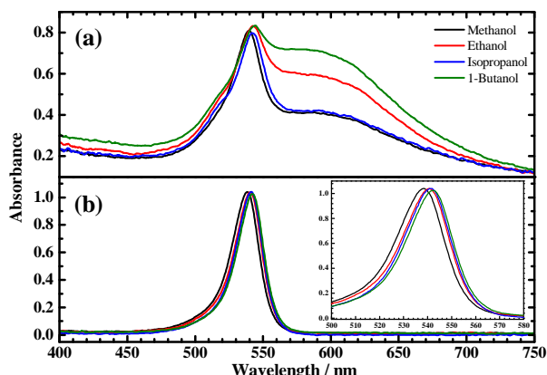
Figure 1-5. Visible absorption spectra of poly(pyrrolyl)squaraines, as synthesized, in hydrogen-bonding solvents: (a) P1 ; (b) P3
