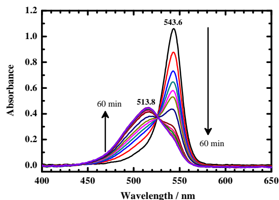
Figure 2-22. Temporal variation of the visible absorption spectrum of poly(3-octylpyrrole)squaraine in trichloromethane solution in a silica cell into which was inserted copper gauze was added to the solution at 296 K: before addition (black curve) and 60 min after addition (purple curve).
