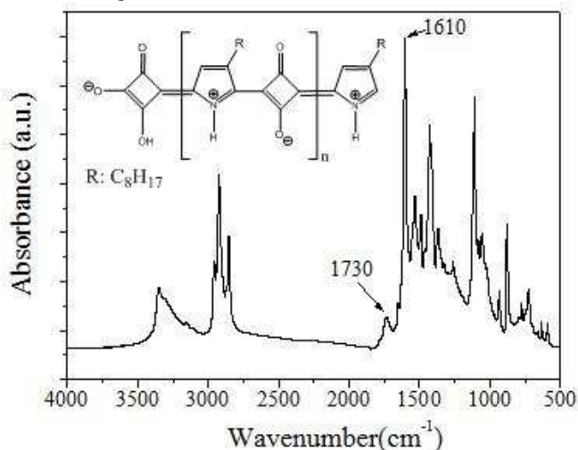
Figure 2. FTIR spectra of PSQ3.
