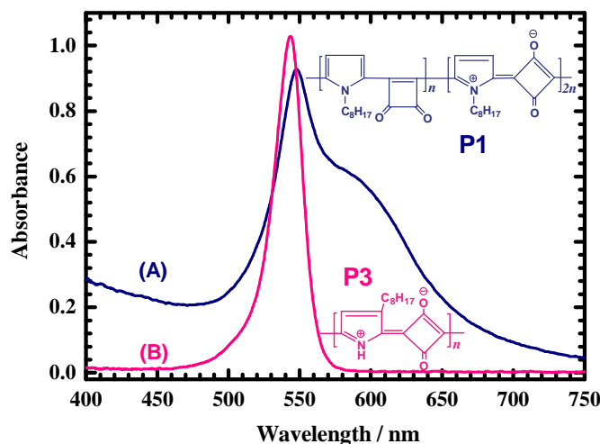
Figure 2-1. Visible absorption spectra of poly(pyrrolyl)squaraines in trichloromethane solution (concentration 3.5 mg/L) and a silica cell (length 1 cm of optical path) at 295 K: (A) poly(1-octylpyrrolyl)squaraine ( P1 ); (B) poly(3-octylpyrrolyl)squaraine ( P3 ). The insets show the molecular structures of P1 and P3 ; P1 consists of repeating units of covalent and zwitterionic structural backbone in a ratio 1:2, whereas P3 possesses mostly zwitterionic repeating units (>97 %).
