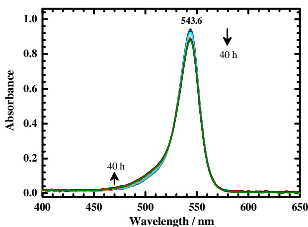
Figure 2-3. Temporal variation over 40 h of visible absorption spectra of poly(3-octylpyrrole)squaraine (3.5 mg/L) in trichloromethane solution (3.0 mL) in a silica cell (optical path 1 cm) into which was inserted a Ag plate (surface area 907 mm 2 ) at 295 K.
