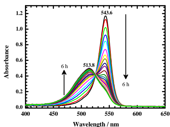
Figure 2-21. Temporal variation of the visible absorption spectra of poly(3-octylpyrrole)squaraine in trichloromethane solution in a silica cell into which was inserted a copper plate (surface area 1720 \text{ mm}^2 ) at 296 K: before addition (black curve) and 6 h after addition (green curve).
