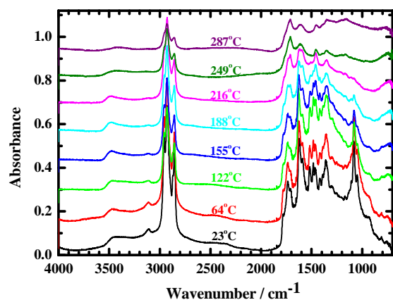
Figure 1-11. IR absorption spectra of P1 at various temperatures as indicated.
