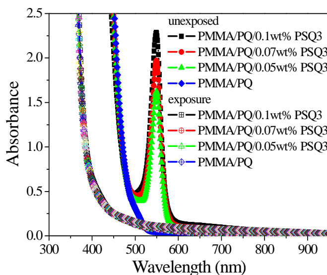
Figure 3. UV–Vis absorption spectra of the unexposed and exposure photopolymers.
