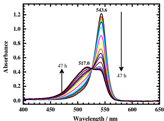
Figure 2-5. Temporal variation over 47 h of visible absorption spectra of poly(3-octylpyrrole)squaraine (3.5 mg/L) in trichloromethane solution (3.0 mL) in a silica cell (optical path 1 cm) into which was inserted Fe plates (surface area 1720 mm 2 ) at 295 K.
