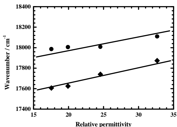
Figure 1-9. Wavenumber of emission maxima of P1 (solid circle) and P3 (solid diamond), as synthesized, versus relative permittivity of methanol, ethanol, isopropanol and 1-butanol.
