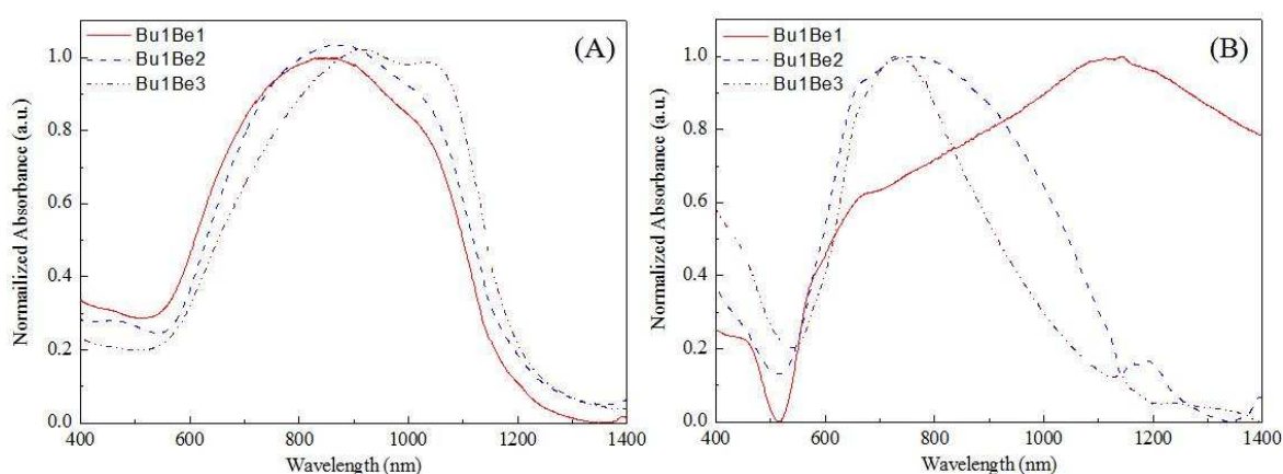
Fig. 7. UV-Vis-NIR spectrum of (A) neat SQI_2 and (B) SQI_5 (after leaching of IL) in three different ratio of n -BuOH/Benzene (Bu/Be) co-solvent, respectively.
