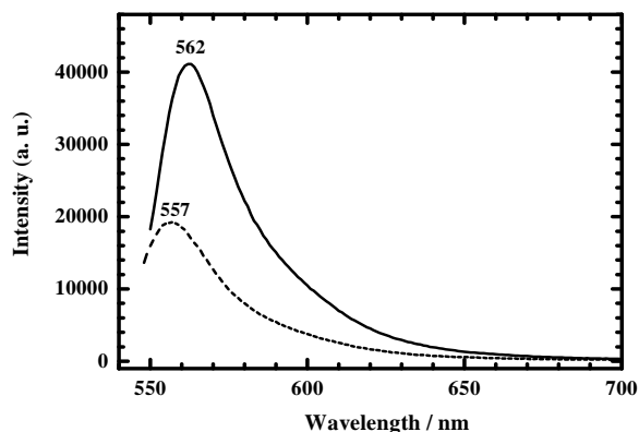
Figure 2-18. Photoluminescent spectra of poly(3-octylpyrrole)squaraine in trichloromethane solution: (solid line) no metal plate, (dashed line) with a Cu plate.
