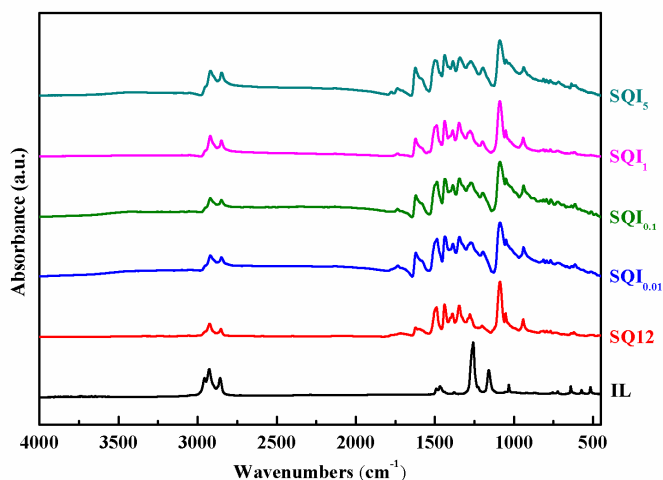
Fig. 2. FT-IR spectra of the neat IL , SQ12 and SQI x .
