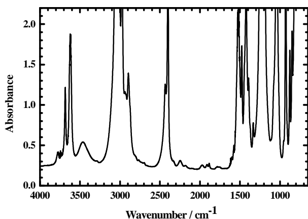
Figure 2-12. IR absorption spectrum of trichloromethane with optical path 1 mm.
