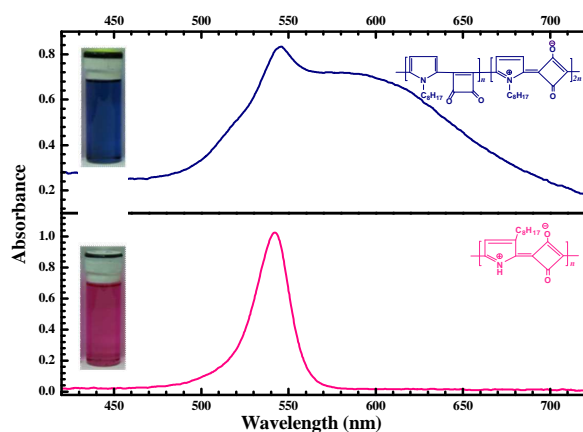
Figure 3-1. The position of the octyl group in the pyrrole derivative affects the construction of the polymer in poly(octylpyrrolyl)squaraine; as a result, visible absorption spectra are reconciled with the backbone structures of poly(octylpyrrolyl)squaraine as synthesized.
