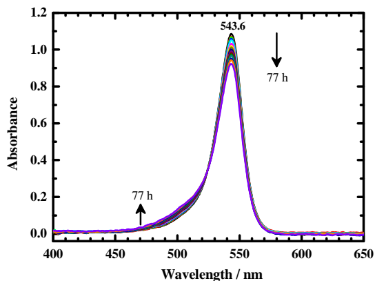
Figure 2-4. Temporal variation over 77 h of visible absorption spectra of poly(3-octylpyrrole)squaraine (3.5 mg/L) in trichloromethane solution (3.0 mL) in a silica cell (optical path 1 cm) into which was inserted a Rh plate (surface area 372 mm 2 ) at 295 K.
