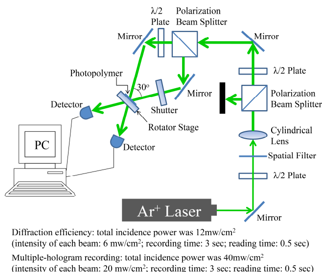
Figure 1. Optical set-up for measuring holographic data recording characteristics.
