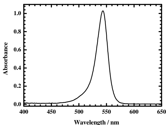
Figure 2-2. Visible absorption spectrum of poly(3-pyrrolyl)squaraines in trichloromethane solution (concentration 3.5 mg/L) and a silica cell (length 1 cm of optical path) at 295 K has no change inserted with metals Al, Co, Ni, Mo, Pd, Sn, Ta, W, Re, Au and stainless steel.
