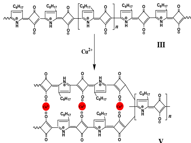
Scheme 2-4. Structural transformation of poly(3-octylpyrrole)squaraine induced by \text{Cu}^{2+} depicted in molecular structures.
