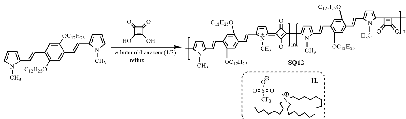
Fig. 1. In the general condensation of aquaric acid with bispyrrole [1]. The IL [Oct 3 NMe][TfO] structure showed within the dotted line.
