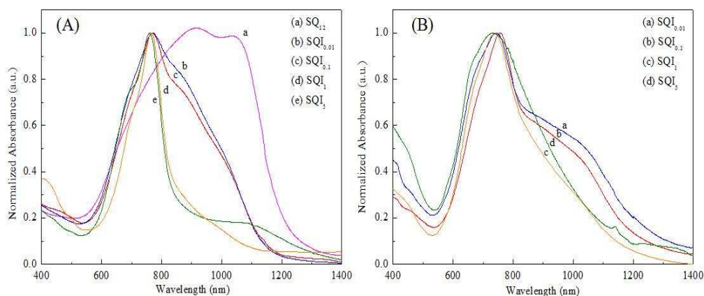
Fig. 5. UV-Vis-NIR spectrum of SQ12 and SQI x in n -BuOH/Benzene(1/3) co-solvent: (A) with IL (B) removing of IL by EtOH.
