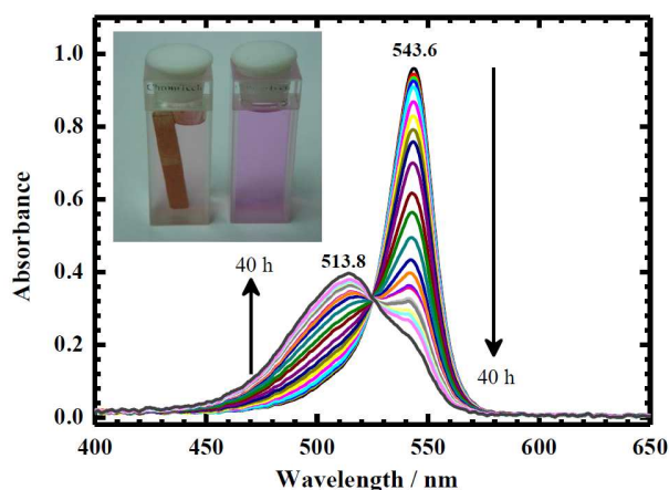
Figure 2-6. Temporal variation over 40 h of absorption spectra of poly(3-octylpyrrole)squaraine in trichloromethane solution in a silica cell into which was inserted a copper plate. Inset photograph: visible color change of poly(3-octylpyrrole)squaraine in \text{CHCl}_3 solution: (right side) no metal plate, (left side) after 40 h with a Cu plate.
