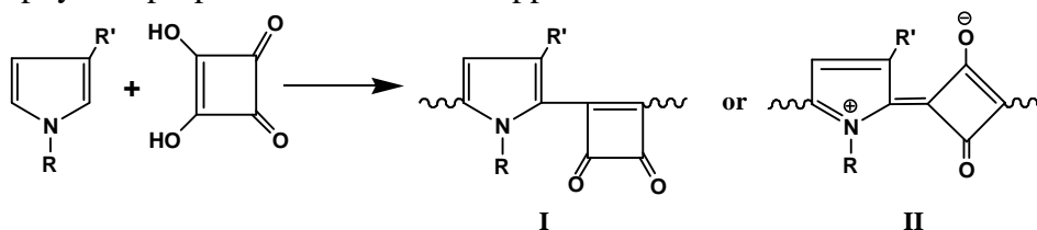
Scheme 1-1. Reaction of a pyrrole derivative with squaric acid in condensation forms repeating units in the structure of poly(pyrrolyl)squaraine of two types, of which formulae I and II imply the covalent and zwitterionic backbones; respectively. R and R' represent H or an alkyl group.
