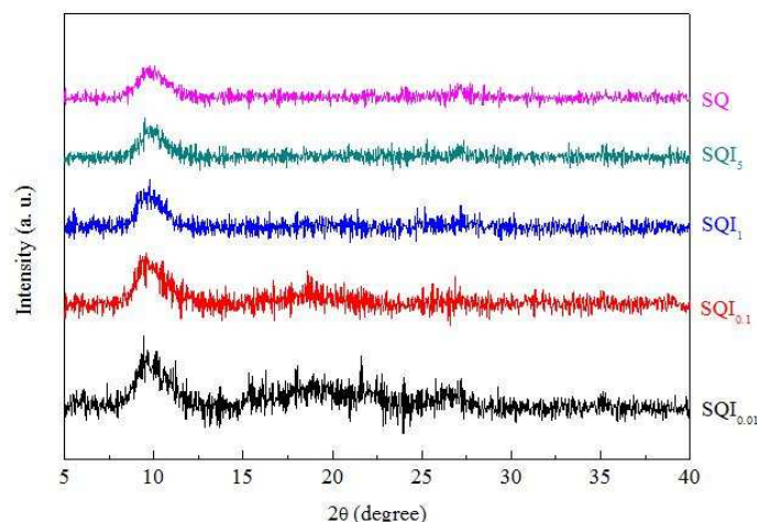
Fig. 4. XRD patterns of polysquaraine: SQ12 and SQI x .
