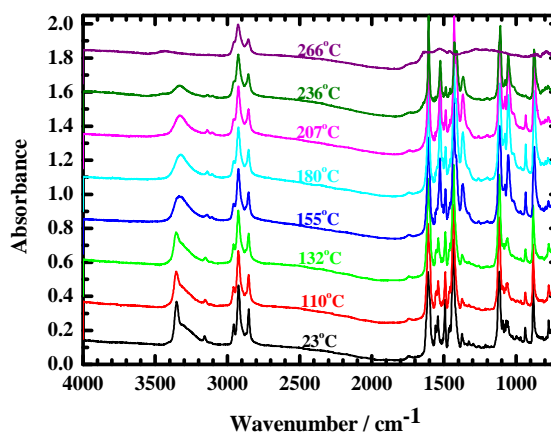
Figure 1-12. IR absorption spectra of P3 at various temperatures as indicated.
