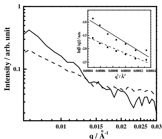
Figure 2-14. SAXS profiles of poly(3-octylpyrrole)squaraine in trichloromethane solution in a copper cell at initial (solid line) and final (dotted line) stages. The inset depicts relations of \ln I(q) versus q^2 for small q at initial (solid line) and final (dotted line) stages.
