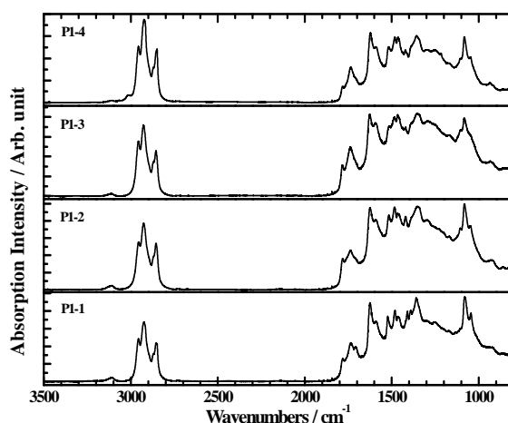
Figure 1-4. IR absorption spectra of polysquaraines P1 as synthesized for four batches.
