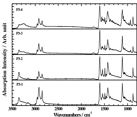
Figure 1-3. IR absorption spectra of polysquaraines P3 as synthesized for four batches.
