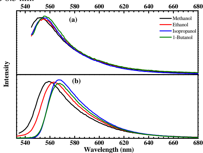
Figure 1-8. Photoluminescence spectra of poly(pyrrolyl)squaraines, as synthesized, in hydrogen-bonding solvents: (a) P1 excited at 540 nm; (b) P3 excited at 530 nm.
