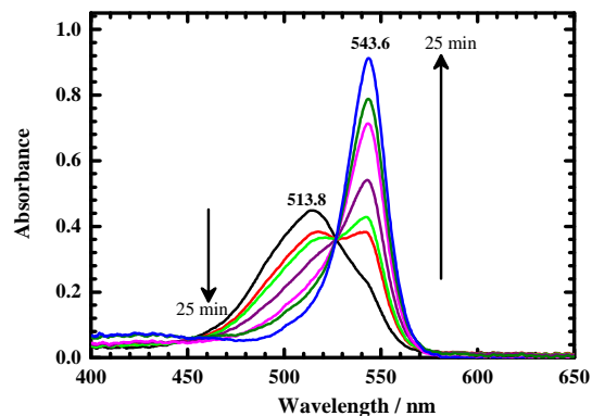
Figure 2-23. Temporal variation of the visible absorption spectrum of poly(3-octylpyrrole)squaraine in trichloromethane in a silica cell after removal of copper plates following ultrasonic agitation (40 kHz, 25 min): before agitation (black curve) and after agitation (blue curve).
