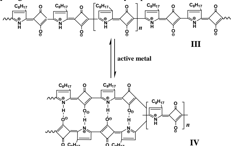
Scheme 2-3. Reversible structural transformation of poly(3-octylpyrrole)squaraine induced by an active metal depicted in molecular structures; formulae III and IV represent the linear and folded conformers, respectively.
