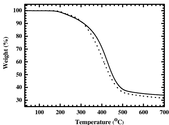
Figure 1-10. Thermal gravimetric analysis (TGA) curves of P1 (solid line) and P3 (dotted line) as synthesized.
