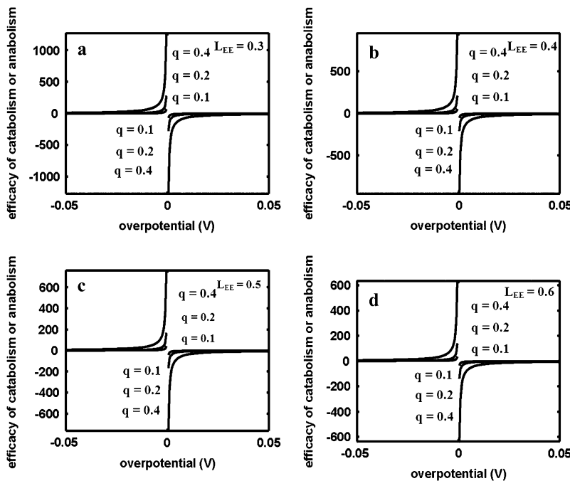
FIGURE 3 Variation of efficacies of catabolism and anabolism under different overpotential, degree of coupling, q , and L_{EE} at static head. \bar{\mu}
