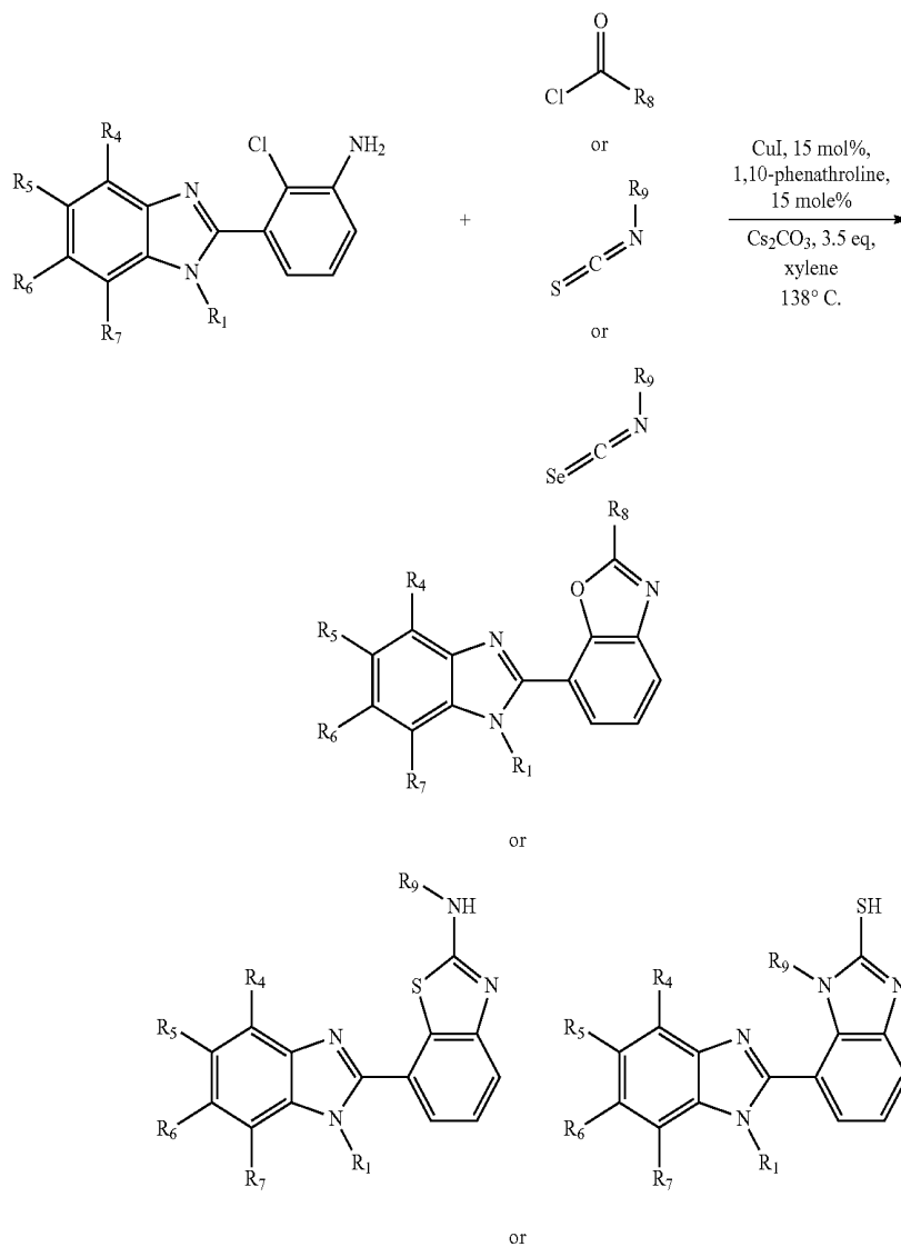
Scheme II
