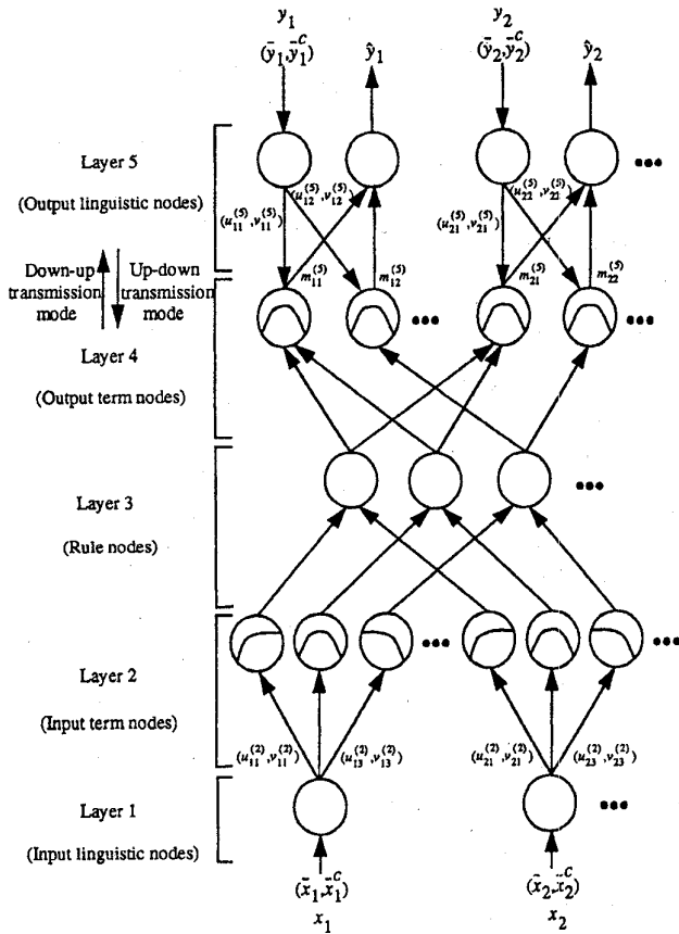
Fig. 3. The proposed FALCON.
