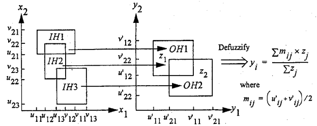
Fig. 5. The fuzzy reasoning process in the FALCON model.
