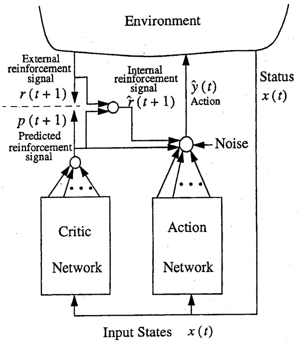
Fig. 6. The proposed RFALCON.
