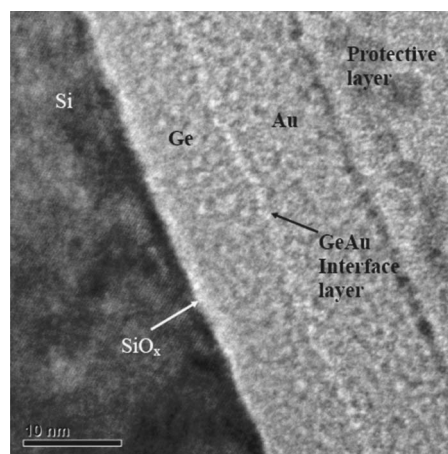
FIG. 6. Cross-sectional view of as-deposited ZnS-SiO x /Ge(8 nm)/Au(8 nm)/Si substrate.
