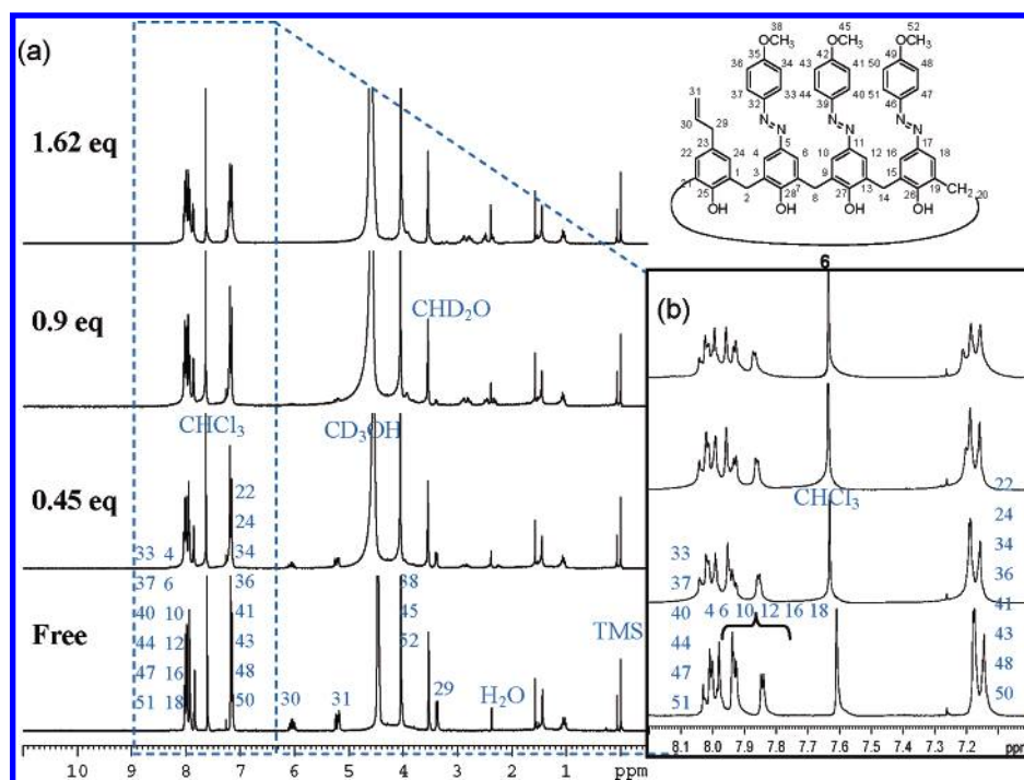
FIGURE 5. (a) ^1\text{H} NMR spectra of compound 6 (5 mM) in a methanol- d_4 /CDCl 3 ( v/v = 1:3 ) cosolvent in the presence of different amounts of \text{Hg}(\text{ClO}_4)_2 . (b) The inset of spectra a in the \delta 7.0–8.2 region.
