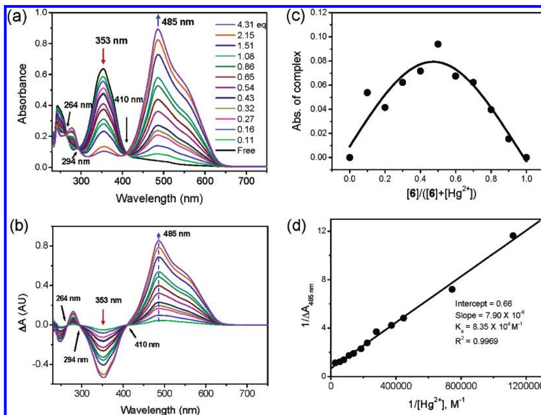
FIGURE 4. (a) UV–vis spectra of 6 ( 8\ \mu\text{M} ) upon titration with \text{Hg}(\text{ClO}_4)_2 in a methanol–chloroform ( v/v = 1/399 ) cosolvent at 25\ ^\circ\text{C} . (b) Difference absorption spectra of a. (c) Job's plot of a 1:1 complex of 6 and \text{Hg}^{2+} ion, where the absorption at 485\ \text{nm} was plotted against the mole fraction of 6 at an invariant total concentration of 10\ \mu\text{M} . (d) Benesi–Hilderbrand plot of 6 with \text{Hg}(\text{ClO}_4)_2 in the same cosolvent system.
