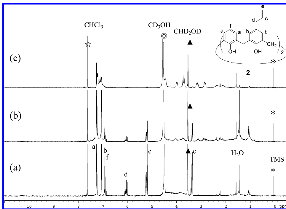
FIGURE 6. (a) ^1\text{H} NMR spectra of compound 2 (5 mM) in a methanol- d_4 /CDCl _3 (v/v = 1:3) cosolvent in the presence of different amounts of Hg(ClO _4 ) _2 : (b) 5.0 and (c) 10 mM.
