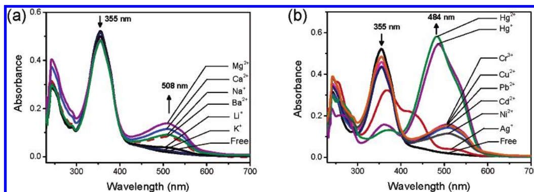
FIGURE 3. UV-vis spectra of 5,11-diallyl-17,23-di( p -methoxyphenyl)azocalix[4]arene 8 ( 10 \mu\text{M} ) before and after adding 9 equiv of various metal perchlorates in a methanol-chloroform ( v/v = 1/399 ) cosolvent at 25^\circ\text{C} : (a) \text{Li}^+ , \text{Na}^+ , \text{K}^+ , \text{Mg}^{2+} , \text{Ca}^{2+} , and \text{Ba}^{2+} and (b) \text{Ag}^+ , \text{Pb}^{2+} , \text{Hg}^{2+} , \text{Cd}^{2+} , \text{Cu}^{2+} , \text{Cr}^{3+} , \text{Hg}^+ , and \text{Ni}^{2+} ions.
