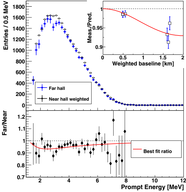
FIG. 4 (color online). The detected energy spectrum of the prompt events of the far-hall ADs (blue) and near-hall ADs (open circle) weighted according to baseline. The far-to-near ratio (solid dot) with the best-fit \theta_{13} value is shown in the lower plot. In the inset is the ratio of the measured to the predicted rates in each AD vs baseline, in which the AD4 (AD6) baseline was shifted relative to that of AD5 by 30 (−30) m.
