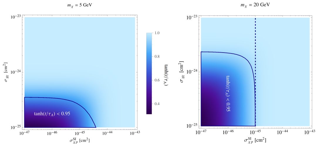
Figure 2. The values of \tanh(t/\tau_A) over \sigma_{\chi p}^{\text{SI}} - \sigma_{\chi\chi} plane at the present day, t = t_{\odot} . The blue-circled area is the non-equilibrium region for N_{\chi} . The vertical line at the right panel indicates the LUX bound, \sigma_{\chi p}^{\text{SI}} \leq 10^{-45} \text{ cm}^2 , for m_{\chi} = 20 \text{ GeV} .
