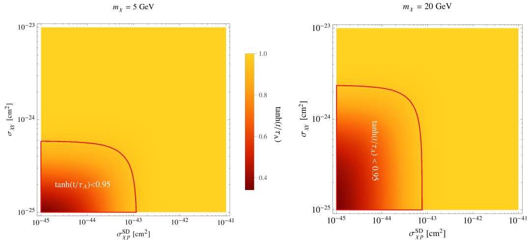
Figure 1. The values of \tanh(t/\tau_A) over \sigma_{\chi p}^{\text{SD}} - \sigma_{\chi\chi} plane at the present day, t = t_{\odot} . The red-circled area is the non-equilibrium region for N_{\chi} .
