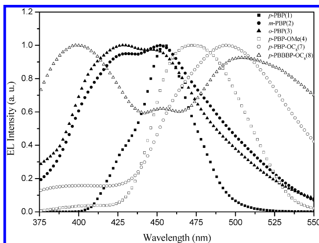
Figure 6. EL spectra of devices PVK:dopant(100:5 by weight)/TPBI(40 nm)/Mg:Ag containing bis(pyridyl) emitters, i.e., p -PBP (1), m -PBP (2), o -PBP (3), p -PBP-OMe (4), p -PBP-OC 8 (7), and p -PBBBP-OC 8 (8).
