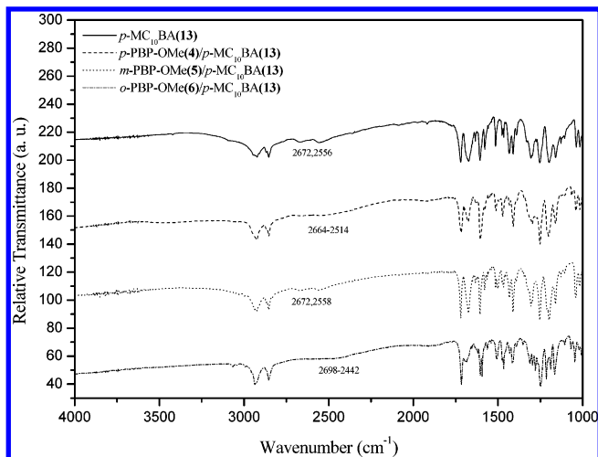
Figure 1. FTIR spectra of donor acid p -MC 10 BA ( 13 ) and its H-bonded trimers containing isomeric pyridyl acceptors, i.e., p -PBP-OMe ( 4 ), m -PBP-OMe ( 5 ), and o -PBP-OMe ( 6 ).
