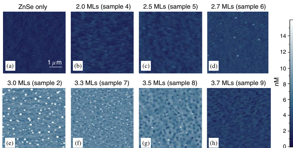
Fig. 2. AFM plane view for samples with the CdSe coverage of (a) 0, (b) 2.0, (c) 2.5, (d) 2.7, (e) 3.0, (f) 3.3, (g) 3.5 and (h) 3.7 MLs, respectively.
