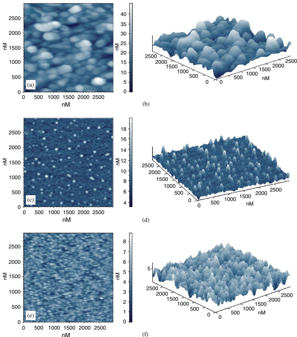
Fig. 1. AFM plane view and three-dimensional view for samples 1 ( T_G = 240 °C), 2 ( T_G = 260 °C) and 3 ( T_G = 280 °C).
