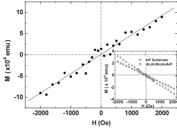
Figure 3. Magnetization as a function of in-plane applied field at 5 K for the (\text{In}_{0.52}\text{Al}_{0.48})_{0.95}\text{Mn}_{0.05}\text{As} epilayer. Closed circles stand for 'net' magnetization after subtracting the magnetization of the InP substrate and the solid line is the results of a linear fit of the experimental data. The inset shows the applied field dependence of magnetization at 5 K for the (\text{In}_{0.52}\text{Al}_{0.48})_{0.95}\text{Mn}_{0.05}\text{As}/\text{InP} substrate and 'bare' InP substrate of the same size.
