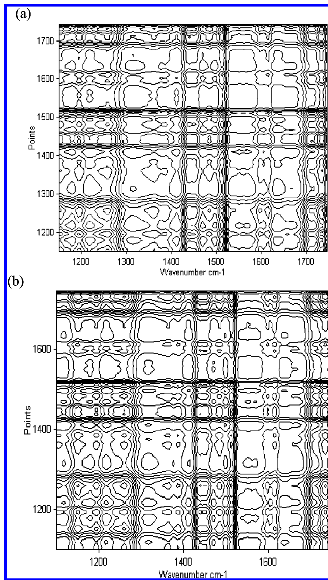
Figure 8. Synchronous 2D correlation map for (a) phenolic/HPMMA blends in the region from 1100 to 1800 \text{cm}^{-1} and (b) phenolic/HPMMA-POSS blends in the region from 1100 to 1800 \text{cm}^{-1} .
