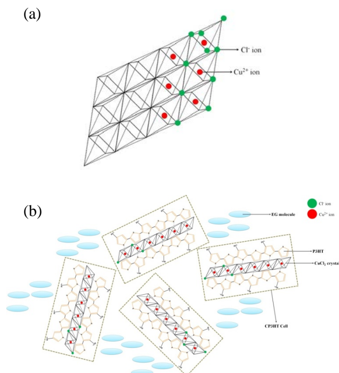
Figure 10: (a) Solid state structure with \text{CuCl}_2 ; \text{Cl}^- ions occupying corner sites and \text{Cu}^{2+} ions occupying interstitial sites. (b) Illustration of the C-P3HT dots dispersed in CE-P3HT.
