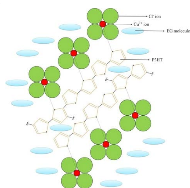
Figure 9: Structural model of the C-P3HT dots dispersed in the complex solution.
