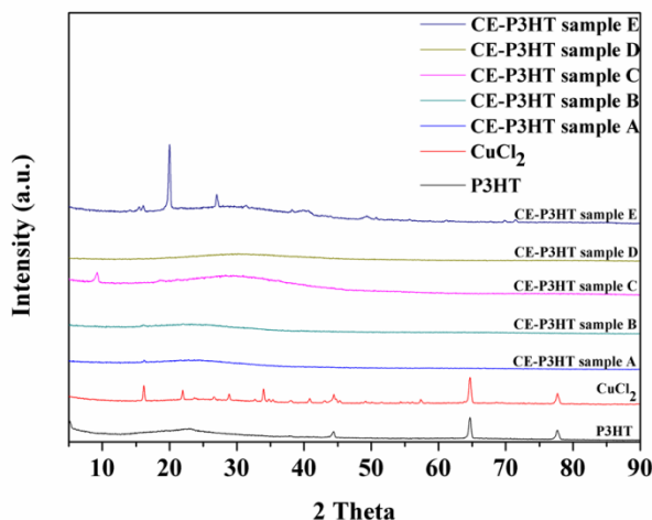
Figure 1: The X-ray spectra of semi-crystalline CE-P3HT samples.
