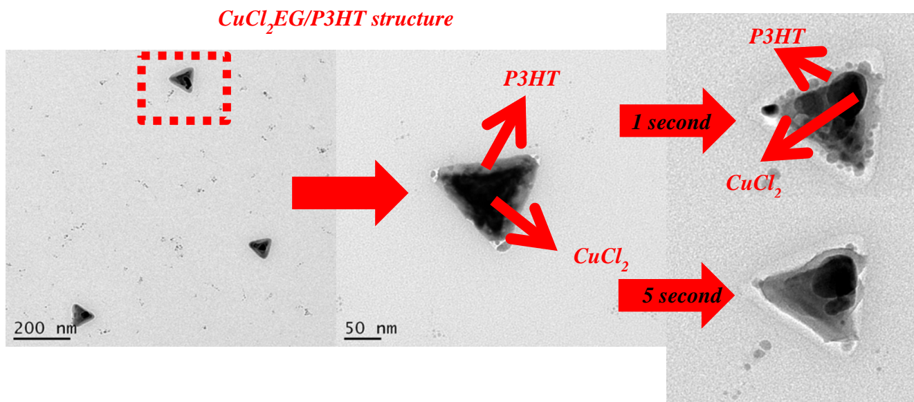
Figure 11: TEM images of CuCl 2 EG/P3HT structure after 1 and 5 second electron beam.
