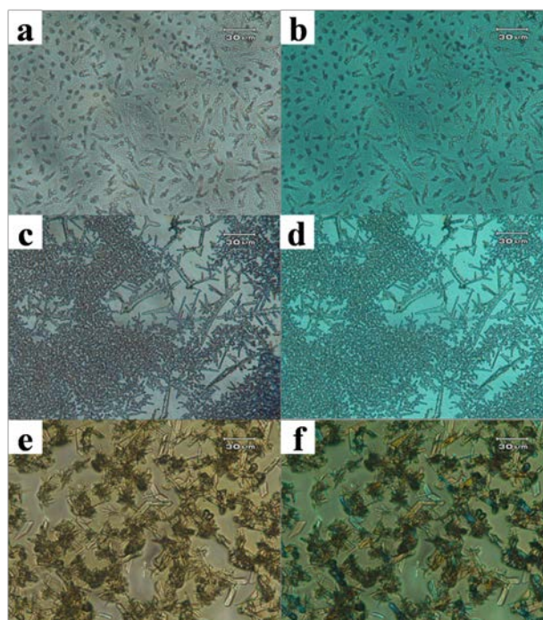
Figure 2: OM images of semi-crystalline CE-P3HT samples, (a) sample C and (b) texture polarized light of sample C, (c) sample D and (d) texture polarized light of sample D, and (e) sample E and (f) texture polarized light of sample E.
