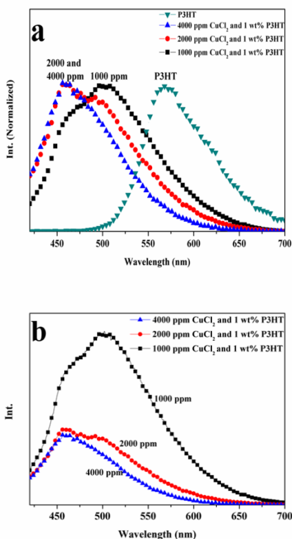
Figure 8: The luminescence of complex solutions, (a) normalized intensity, (b) relative intensity.
