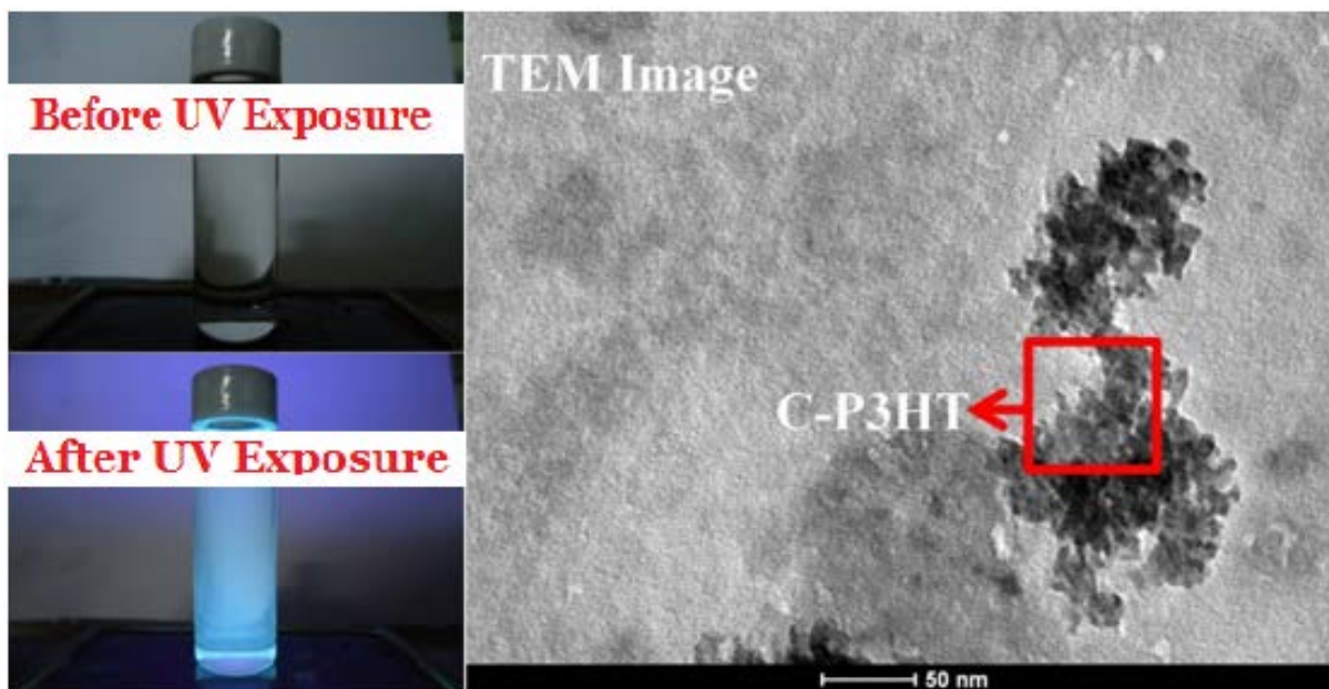
Figure 6: The phenomenon of dispersed C-P3HT in complex solution and semi-crystalline CE-P3HT F, formed with 250 ppm CuCl 2 EG and 4 wt% P3HT.
