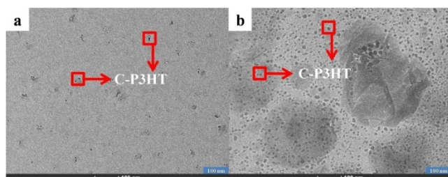
Figure 4: TEM images of C-P3HT, derived from (a) CE-P3HT sample C, and (b) CE-P3HT sample E.
