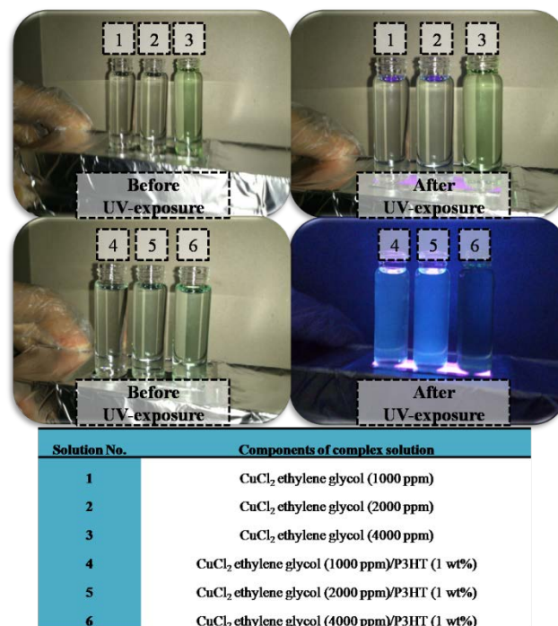
Figure 5: Photographs of complex solutions and pure \text{CuCl}_2 EG solutions under with and without UV illumination (wavelength: 254 nm).
