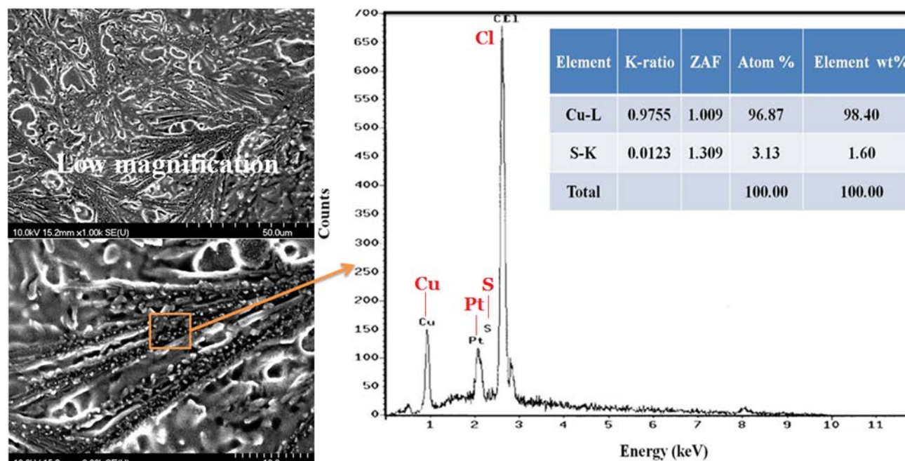
Figure 3: The SEM and EDS images of semi-crystalline CE-P3HT sample C.
