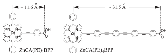
Fig. 1 Structures of carboxyphenylethynyl zinc porphyrins. Distances are measured from zinc(II) ions to the carbon of the carboxylic group of the ZINDO-optimized structures.
