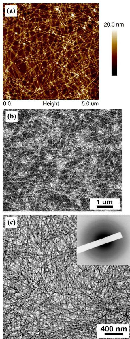
Figure 1 (a) AFM (b) SEM and (c) TEM images of P3HT NWs. Inset in (c) shows the selected area electron diffraction pattern of the P3HT NWs. 418x1014mm (96 x 96 DPI)
