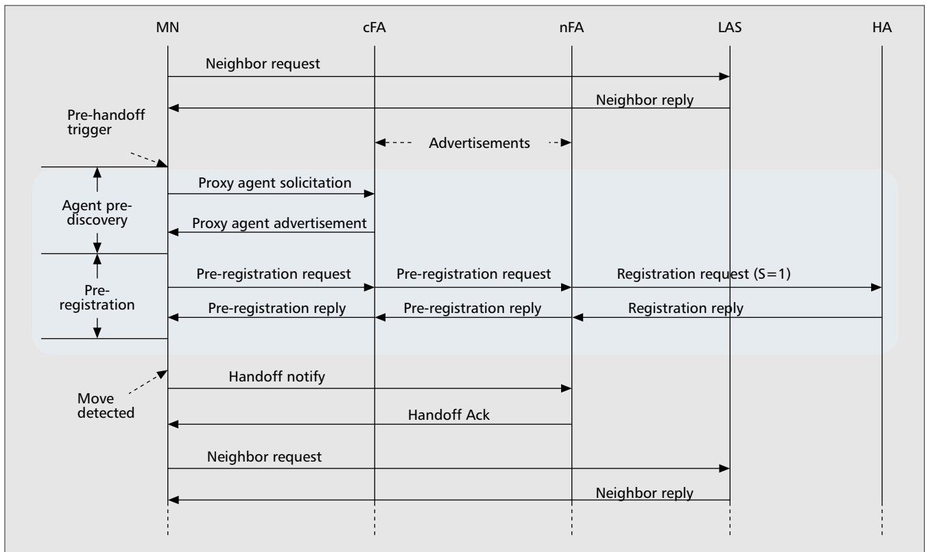
■ Figure 3. Message flow for the FA-CoA case.
