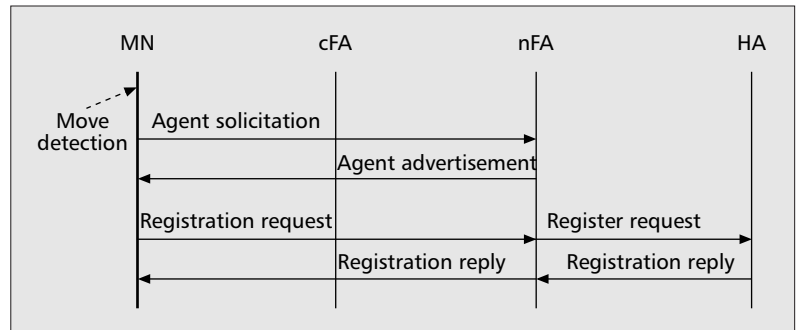
■ Figure 1. Mobile IP handoff in the FA-CoA case.
