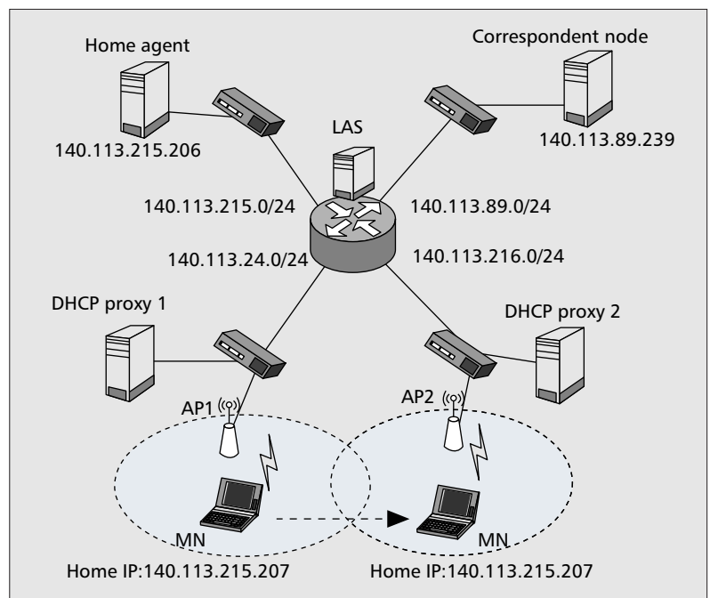
■ Figure 5. Experimental setup.
