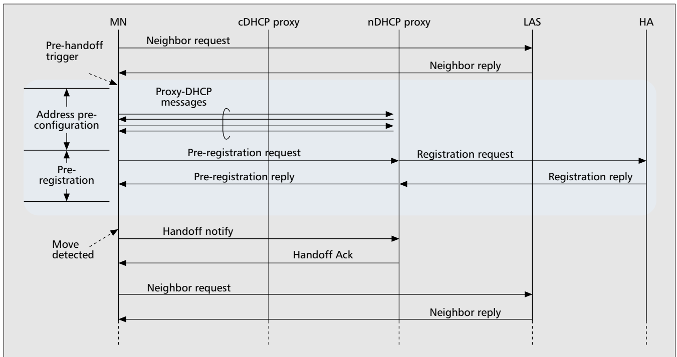
■ Figure 4. Message flow for the CCoA case.
