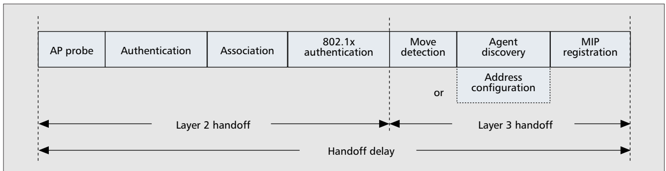
■ Figure 2. Total handoff delay.
