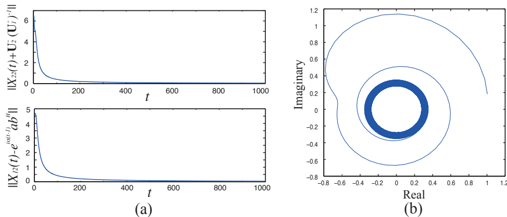
FIG. 2. Set \alpha = 1.771 , n_1 = 2 , n_2 = 1 , and \beta = 1 . (a) \|X_{22}(t) + \mathbf{U}_2^-(\mathbf{U}_1^-)^{-1}\| and \|X_{12}(t) - e^{i\alpha(t-1)}ab^H\| with a = X_{12}^1(W_2^-)^{-1}e_n and b = (\mathbf{U}_1^-)^{-H}e_n are plotted for 1 \leq t \leq 10^3 . (b) Phase portrait of the (1, 1) entry of X_{12}(t) is plotted for 1 \leq t \leq 10^3 .
