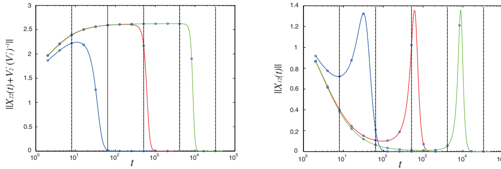
FIG. 1. \|X_{22}(t) + V_2^-(V_1^-)^{-1}\| and \|X_{12}(t)\| are plotted for 1 \leq t \leq 1.5 \times 10^4 with r = 0.1 (blue line), 0.01 (red line), and 0.001 (green line).
