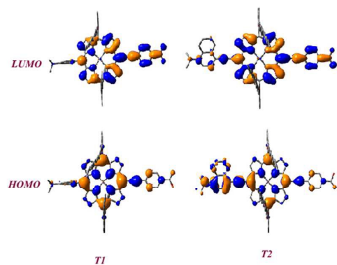
Figure 3. Frontier molecular orbitals of T1 and T2
