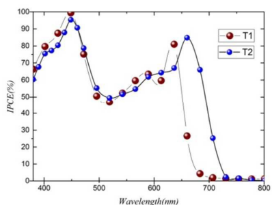
Figure 5 The IPCE action spectra for DSSCs based on T1 and T2
