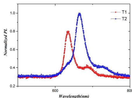
Figure 2. Fluorescence spectra of T1 and T2 in ethanolic solution (0.5mM) at 460 \text{ nm} excitation wavelength
