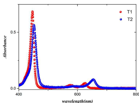
Figure 1-Uv-Vis spectra of T1 and T2 in ethanolic solution (0.5mM)
