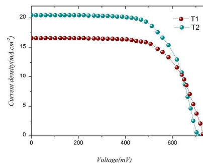
Figure 4. The current-voltage (J-V) characteristics of T1 and T2
