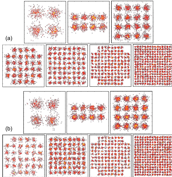
Fig. 5. Measured corresponding constellations of OFDM signal with bit-and-power-loading algorithm at the bias currents of (a) 4 and (b) 3.5 mA.
