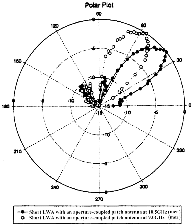
Fig. 7. The measured radiation patterns of the short LWA integrated with an aperture-coupled patch antenna at 9.0 and 10.5 GHz.
