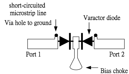
Fig. 3. Schematic diagram of the varactor-tuned phase shifter.
