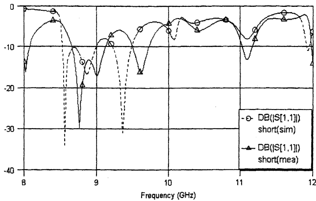
Fig. 4. Simulated and measured return loss of the short LWA with an open end.
