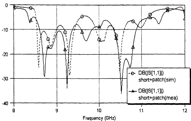
Fig. 5. Simulated and measured return loss of the short LWA integrated with an aperture-coupled patch antenna.
