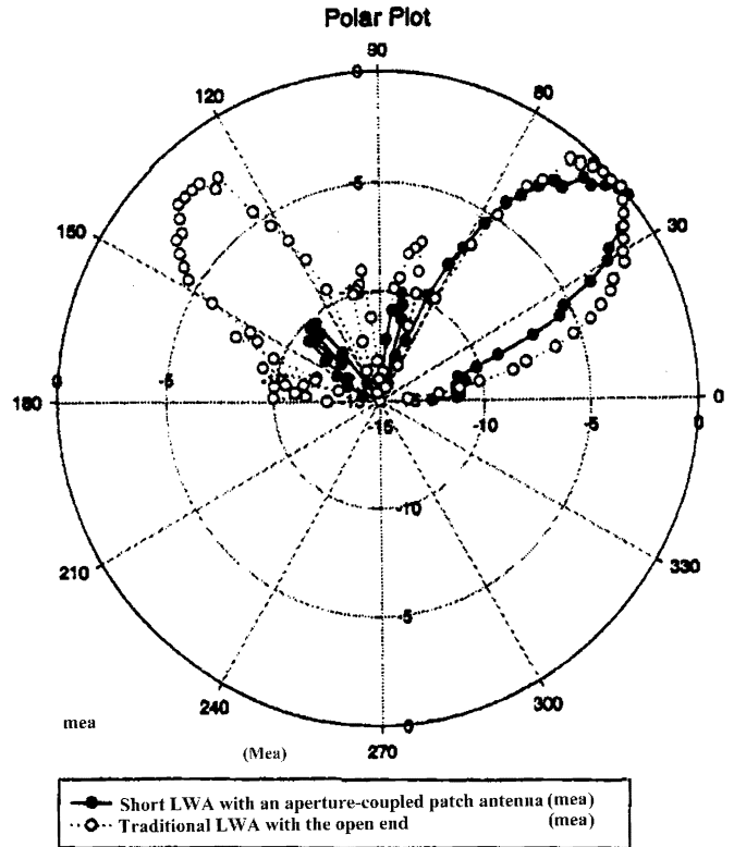
Fig. 6. Comparison of the measured H-plane radiation patterns of the proposed antenna structure comparing to the traditional LWA at 10.5 GHz.
