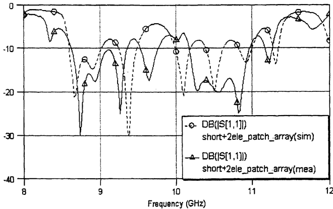
Fig. 8. The simulated and measured return loss of the short LWA integrated with 2-element aperture-coupled patch antenna arrays.
