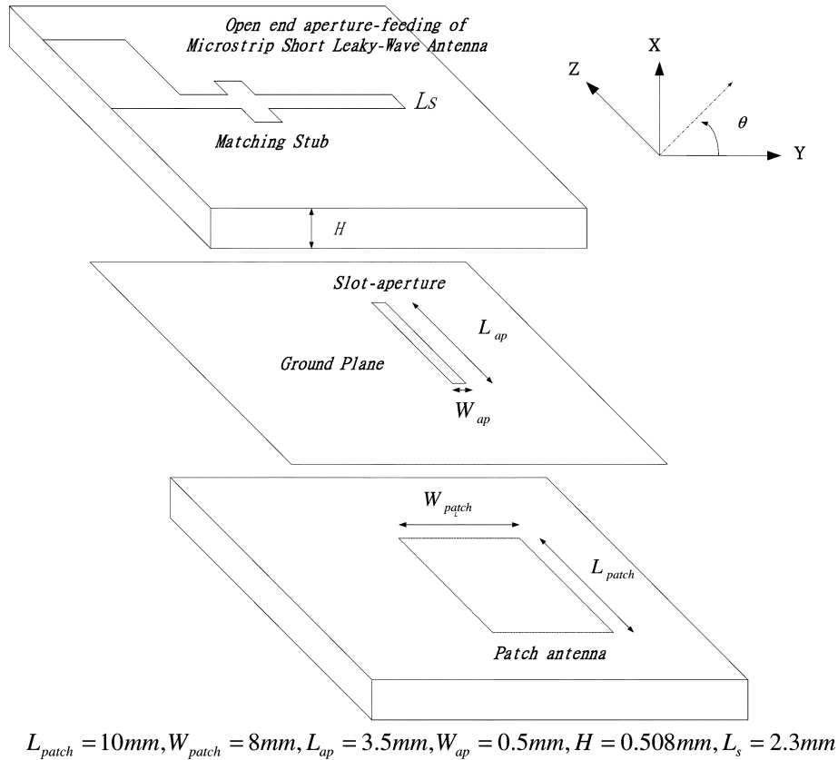
Fig. 2. Geometry and coordinate system for the aperture-coupled patch antenna.
