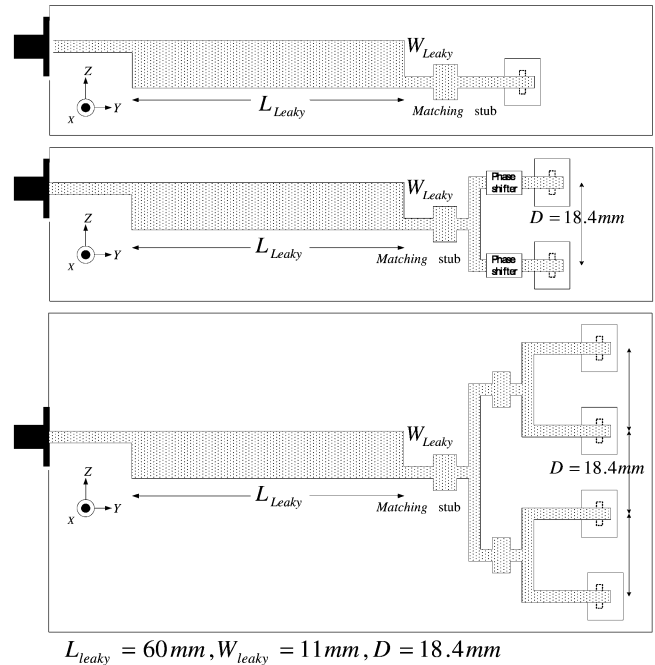
Fig. 1. Configuration of the short leaky-wave antenna integrated with the 1-, 2-, and 4-element aperture-fed patch antenna arrays.
