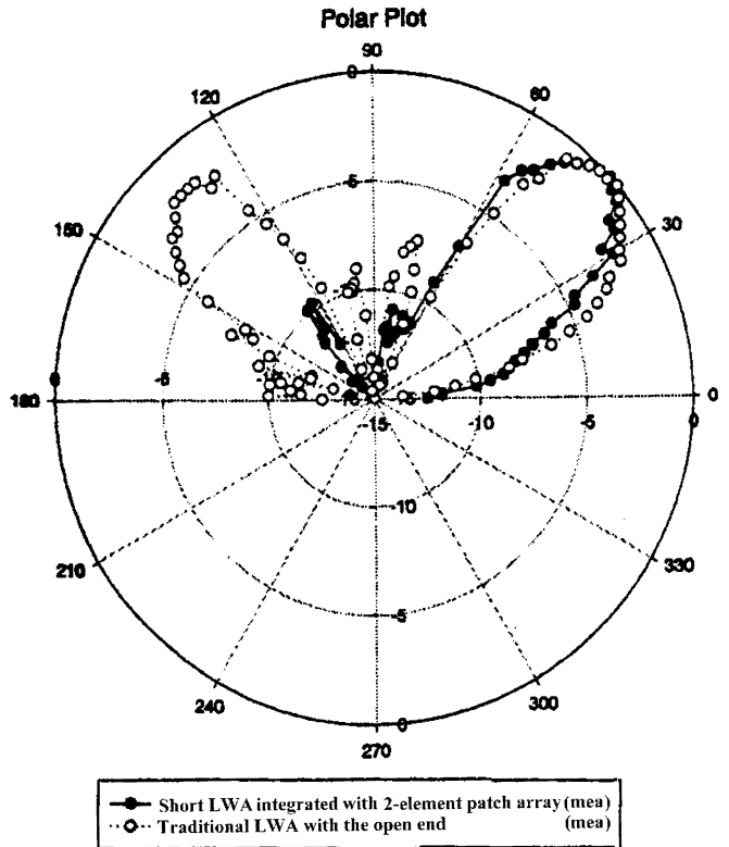
Fig. 10. Comparison of the measured radiation patterns between the short LWA integrated with the 2-element aperture-coupled patch arrays and the traditional LWA.
