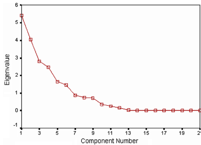
Fig. 2. Scree plot and factor analysis of transportation mode-choice criteria.
