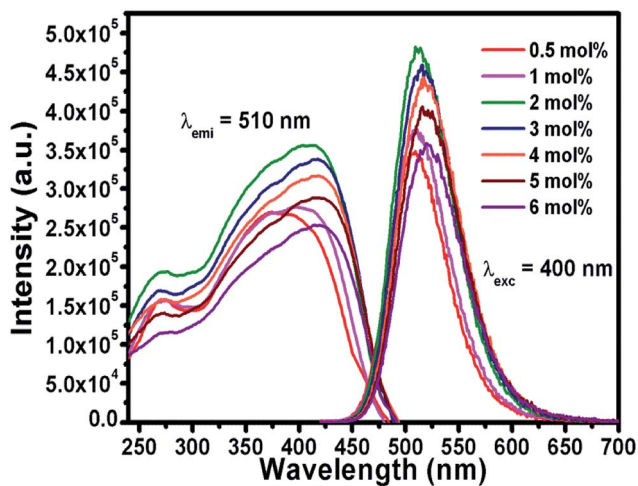
Fig. 4 PLE and PL spectra of BSOC:Eu 2+ phosphor with the variation of Eu 2+ concentration.
