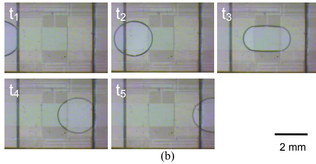
Fig. 9 Interface tests. (a) Electrical states for control electrodes at each period. (b) Continuous images for droplet passing through the connector. The electrode is 1500 \mu\text{m} wide, the droplet is 2.5 \mu\text{l} DI water, and the applied voltage is 80 V_{AC} , 2 kHz sine wave.
