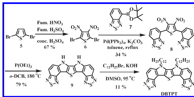
Scheme 2. Synthesis of Fused A-D-A DBTPT
