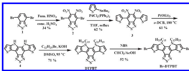
Scheme 1. Synthesis of Fused D-A-D Pentacyclic Structure DTPBT
