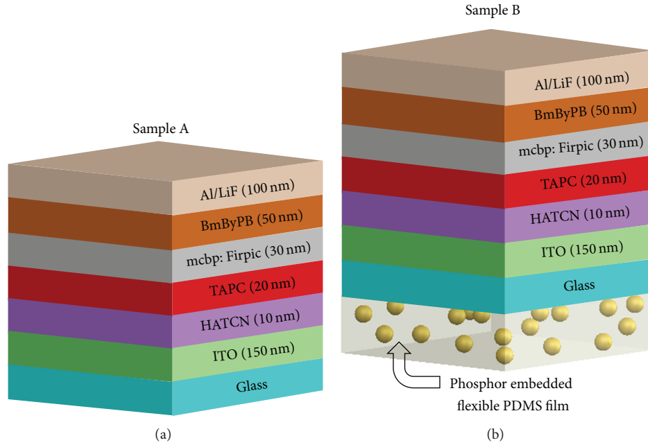
FIGURE 1: Schematic structures of OLEDs device (a) without a yellow phosphor embedded flexible film as a reference and (b) with a yellow phosphor embedded flexible film.
