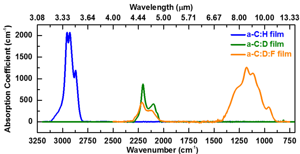
Figure 3. FTIR spectra of the host a-C:H, a-C:D, and a-C:D:F ( \text{CF}_4/[\text{CF}_4 + \text{CD}_4] = 50 vol.%) films without Yb metal-organic compound incorporation prepared under the same deposition condition except for the precursor gas. The relative wavenumber/wavelength positions and the range of the first vibrational mode illustrated in Figure 2 are inferred from this data.
