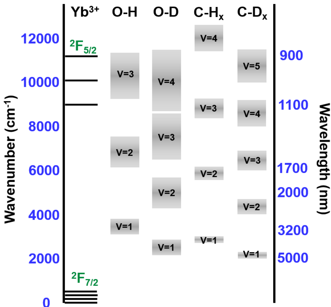
Figure 2. Illustration of energy levels of the vibrational modes for O–H, O–D, C–H x , and C–D x bonds in the solid state, where the range of each vibrational mode is inferred from Fourier transform infrared spectroscopy (FTIR) spectra of the host a-C:H, a-C:D and fluorinated a-C:D films (a-C:D:F) as displayed in Figure 3. The grey band here is used to represent the highly varying bonding structure, which reflects the levels associated with the numerous combinations of nearest neighbors and the different local bonding environments.
