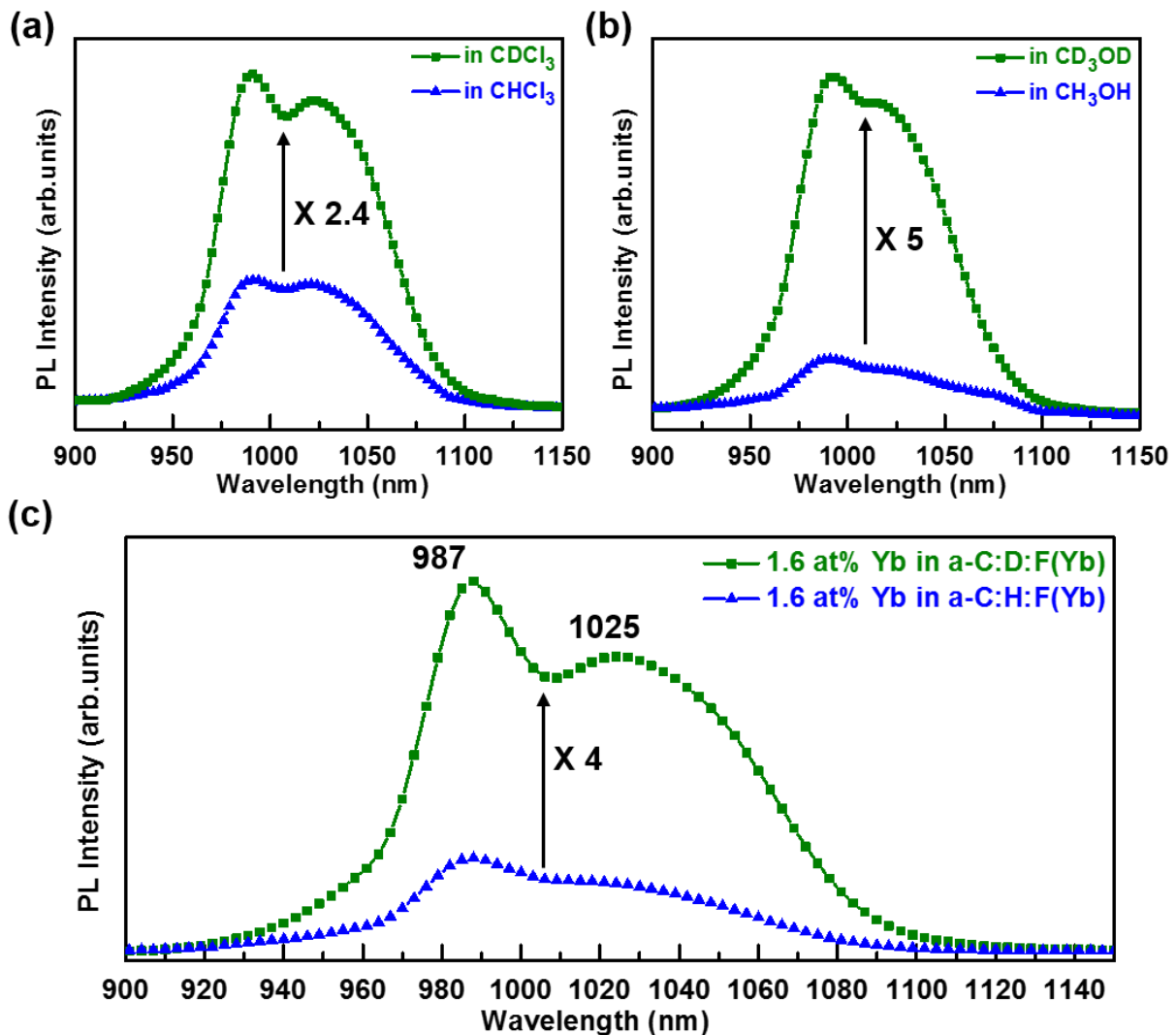
Figure 1. Comparison of the Photoluminescence (PL) intensity of \text{Yb}(\text{fod})_3 powder dissolved in (a) chloroform ( \text{CHCl}_3 ) and chloroform-d ( \text{CDCl}_3 ); in (b) methanol ( \text{CH}_3\text{OH} ) and methanol-d 4 ( \text{CD}_3\text{OD} ); (c) Comparison of the PL intensity of a-C:D:F(Yb: 1.6 at %) and a-C:H:F(Yb: 1.6 at %) films prepared using RF power of 60 W, precursor gas flow rate of 20 sccm, deposition pressure of 60 mTorr, substrate temperature of 90 °C, and \text{Yb}(\text{fod})_3 powder evaporation temperature of 110 °C.
