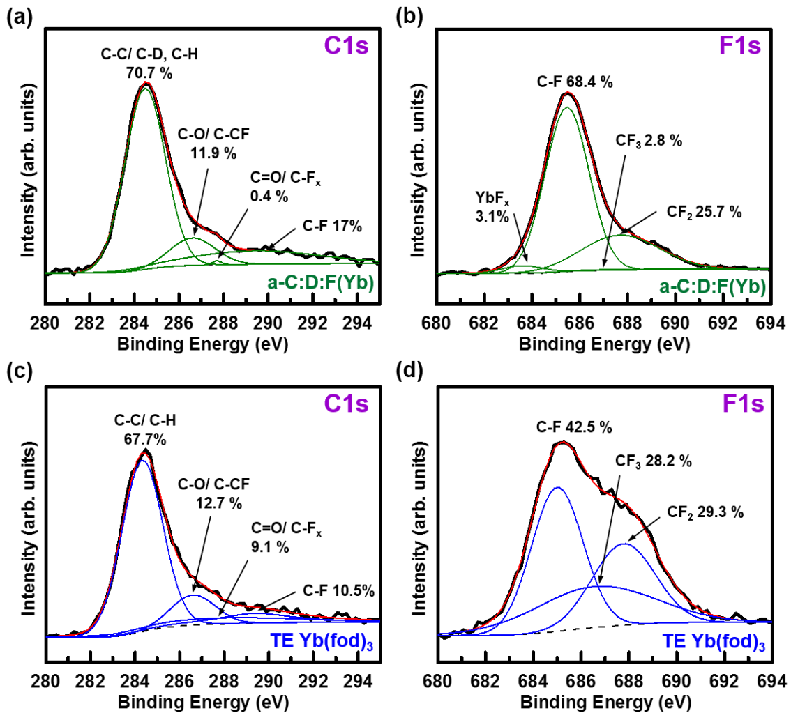
Figure 5. Deconvoluted XPS (a) C1s and (b) F1s spectra of the a-C:D:F(Yb) film with maximum I_{\text{nor}} prepared using RF power of 60 W, precursor gas flow rate of 20 sccm, deposition pressure of 60 mTorr, substrate temperature of 80 °C, and Yb(fod) 3 powder evaporated at a temperature of 110 °C; and (c) C1s and (d) F1s spectra of the TE Yb(fod) 3 film.
