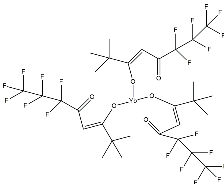
Figure 6. Illustration of the Yb metal-organic compound, Yb(fod) 3 , with chemical structure Yb(C 10 H 10 O 2 F 7 ) 3 .
