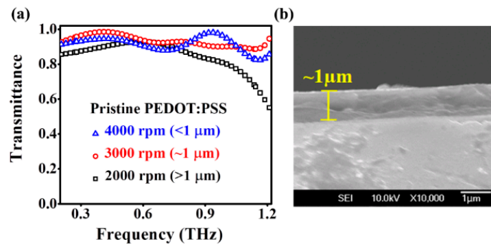
Figure 3. (a) THz transmittance of pristine PEDOT: PSS layers with three different thicknesses controlled by the rotation speed of the spin coater and (b) FESEM cross-sectional image of the 1 \mu\text{m} thick pristine PEDOT: PSS layer deposited on clean substrate by spin coating with a rotation speed of 3000 rpm for 30 s.
