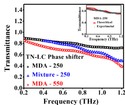
Figure 8. THz transmittance of three types of TN-LC phase shifters at 0 V_{RMS} . The experimental data (symbol) are verified by theoretical calculation (solid line), as shown in the inset.
