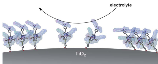
Scheme 3 Schematic illustration of a possible model of LD16 assembly on \text{TiO}_2 . The colour surfaces represent the long alkoxy/alkyl chains of LD16. Note that the surface of \text{TiO}_2 is not completely covered by LD16 to represent the experimental conditions in Fig. 3c. This scheme implies that the alkoxy/alkyl chains could form a hydrophobic layer between the electrolyte and \text{TiO}_2 when the dyes fully cover the \text{TiO}_2 surface.
