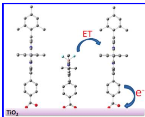
Scheme 2. Proposed Alignments of Porphyrin Dye and BET on the Surface of TiO 2 and Energy Transfer Pathway
