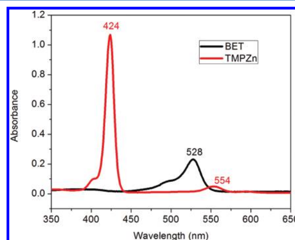
Figure 2. Absorption spectra of the TMPZn and the BET in \text{CH}_2\text{Cl}_2 at room temperature. The concentration of dyes was 2 \times 10^{-6} mol/L.
