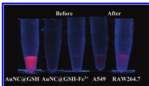
Figure 5. Luminescence switched-on assays of the cell lysate samples. The vial on the left-hand side is the \text{AuNCs@GSH} solution (0.5 mM). The two vials containing \text{AuNCs@GSH-Fe}^{3+} are labeled “Before.” After adding the cell lysate samples to these two vials and incubating for 30 min, the resultant vials were labeled “After.” The cell lysate samples ( 10\ \mu\text{L} , 10^6 cells/mL) included human lung adenocarcinoma epithelial A549 cell line (A549) and RAW264.7 macrophages. The switch-off solution ( \text{AuNCs@GSH-Fe}^{3+} ) was prepared by mixing the \text{AuNCs@GSH} (0.5 mM, 40\ \mu\text{L} ) and aqueous \text{FeCl}_3 (2.5 mM, 10\ \mu\text{L} ) for 15 min.
