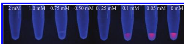
Figure 1. Photograph of the AuNCs@GSH (10 μL, 0.756 mM) (under illumination of UV light, λ max = 365 nm) following incubation with different concentrations of FeCl 3 solution (10 μL). The concentrations indicated on the figure refers to the initial concentrations of Fe 3+ prior to mixing.
