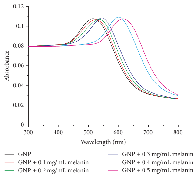
FIGURE 7: UV spectra for the titration of 17 nm GNP with melanin. Melanin is mixed with GNP at final concentrations of 0, 0.1, 0.2, 0.3, 0.4, and 0.5 mg/mL for melanin and 0.34 mM for GNP. UV absorbance of the binding reactions is shown. Red-shift of the absorbance peak indicates the increasing diameter of binding complex.
