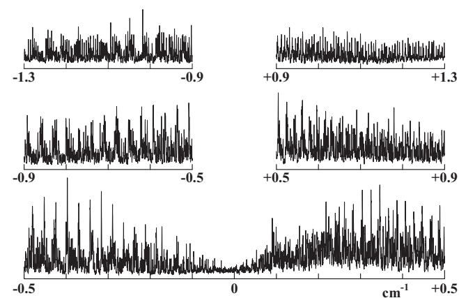
FIG. 6. Rotationally resolved fluorescence excitation spectrum of the S_1 \ ^1B_{3u} \leftarrow S_0 \ ^1A_g \ 0_0^0 transition of pyrene- h_{10} .
