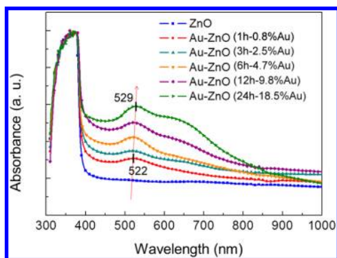
Figure 2. Absorption spectra of Au–ZnO photoelectrodes with Au nanoparticles deposited over various periods.
