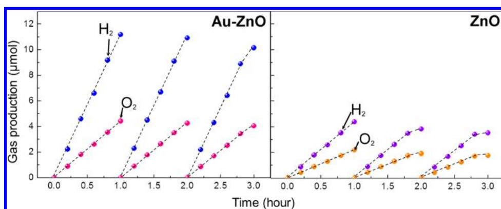
Figure 9. Time courses of H 2 and O 2 evolution using Au–ZnO and ZnO photoelectrodes under AM 1.5G solar simulator in 0.5 M Na 2 SO 4 aqueous solution.
