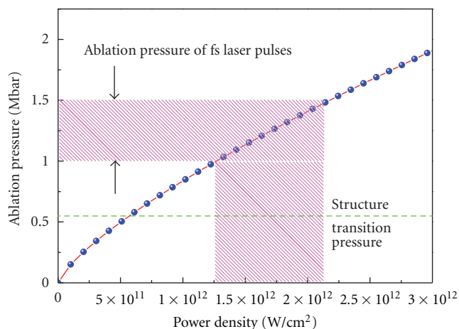
FIGURE 3: Simulated ablation pressure as a function of the laser peak power density according to (3). The shadow area indicates the range of laser peak power density in this study and corresponding ablation pressure. The dashed line represents the pressure of zinc blende-wurtzite phase transition, that was obtained from [28].
