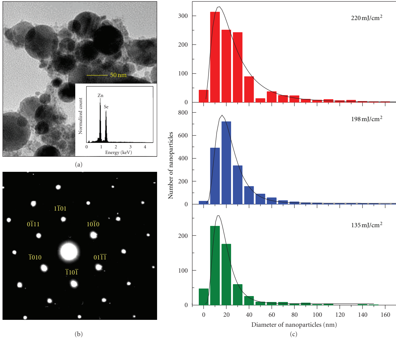
FIGURE 1: (a) TEM images of ZnSe nanoparticles fabricated by the fluence of 220 mJ/cm 2 . Inset: the EDS spectrum shows the composition of ZnSe nanoparticles. (b) TEM diffraction patterns of ZnSe nanoparticles in (a). (c) Size distribution of ZnSe nanoparticles at various laser fluences corresponding to the TEM images in (a) with an area of 3.2 \mu\text{m} \times 2.6 \mu\text{m} . The solid lines are the log-normal fitting.
