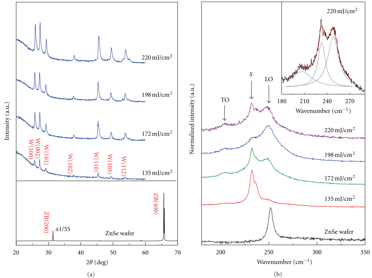
FIGURE 2: (a) X-ray diffraction patterns of ZnSe wafer and ZnSe nanoparticles fabricated at various laser fluences. W: Wurtzite. ZB: Zinc blende. (b) Raman spectra of ZnSe wafer and ZnSe nanoparticles fabricated at various fluences. The 633.0 nm laser was used as the excitation light. Inset: the Raman spectra of ZnSe nanoparticles fabricated at fluence of 220 mJ/cm 2 on a large scale with Lorentz peak fitting. TO: transverse optical phonon mode. LO: longitudinal optical phonon mode. S: surface phonon mode.
