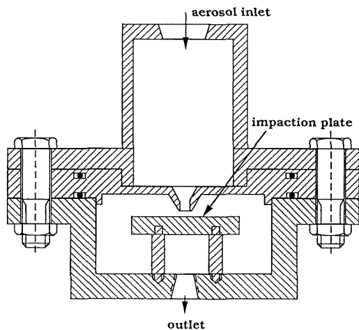
FIGURE 1. A schematic drawing of the present impactor.
