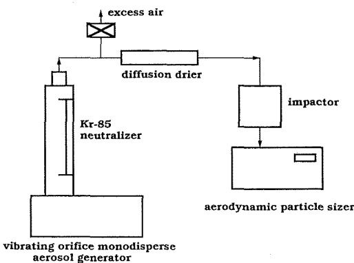
FIGURE 3. Schematic diagram of the present experimental setup.
