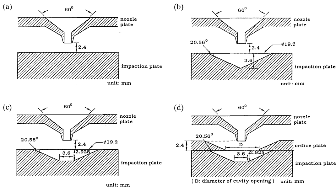
FIGURE 2. Various impaction surface designs. (a) Design No. 1. (b) Design No. 2. (c) Design No. 3. (d) Design No. 4.
