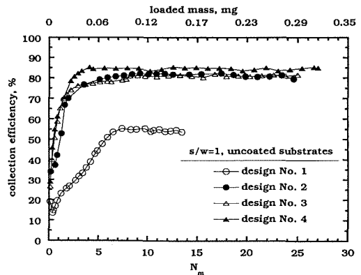
FIGURE 6. Collection efficiency versus N_m and loaded particle mass for uncoated impaction surfaces. D_{pa} = 3.2 \pm 0.04 \mu\text{m} ; total running time = 90 min.
