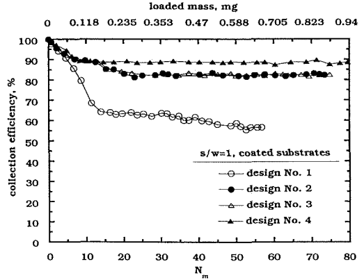
FIGURE 4. Collection efficiency versus N_m and loaded particle mass for coated impaction surfaces. D_{pa} = 3.4 \pm 0.05 \mu\text{m} ; total running time = 120 min.
