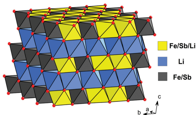
Fig. 3 Polyhedral presentation of the \text{Li}_4\text{FeSbO}_6 crystal structure. Note that mixed site occupancies are largely fictitious, as discussed in the text.
