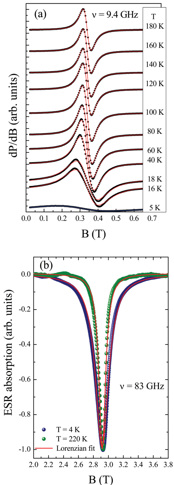
Fig. 15 Temperature evolution of the first derivative absorption line (a) and full ESR absorption (b) for \text{Li}_4\text{FeSbO}_6 antimonate at two different frequencies: points – experimental data, lines – fitting in accordance with the Lorentzian profile (eqn (10)).
