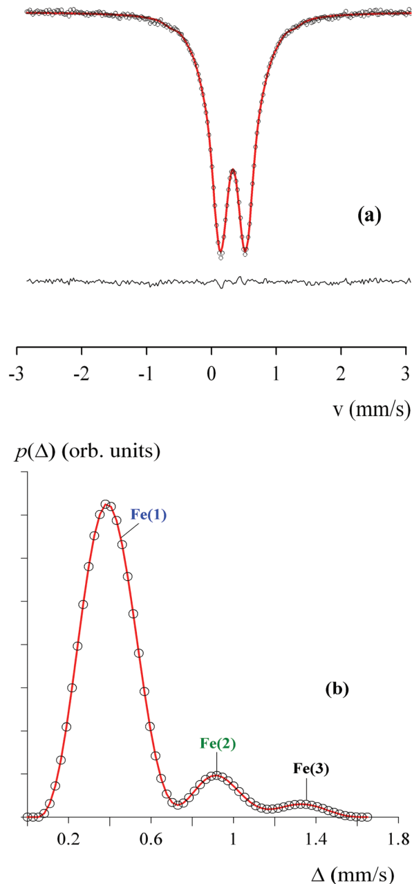
Fig. 4 The ^{57}\text{Fe} Mössbauer spectrum of the sample \text{Li}_4\text{FeSbO}_6 recorded at T = 300\text{ K} (a); distribution functions of the quadrupole splitting p(\Delta) (b).
