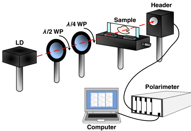
Fig. 1 Experimental setup. \lambda/2 WP and \lambda/4 WP represent half- and quarter-waveplates. LD is a laser diode, and the header is an optical detector.
