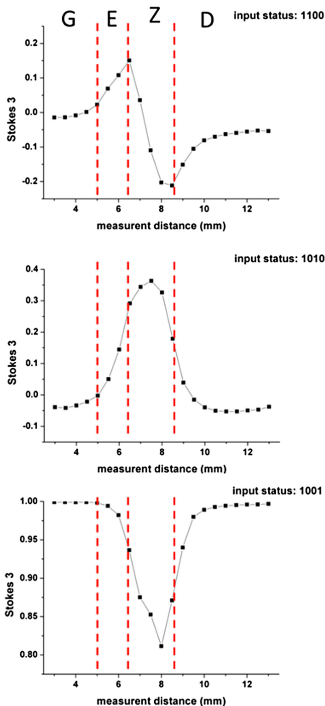
Fig. 6 Stokes 3 of three input states (horizontal, +45 deg, right circular polarization).
