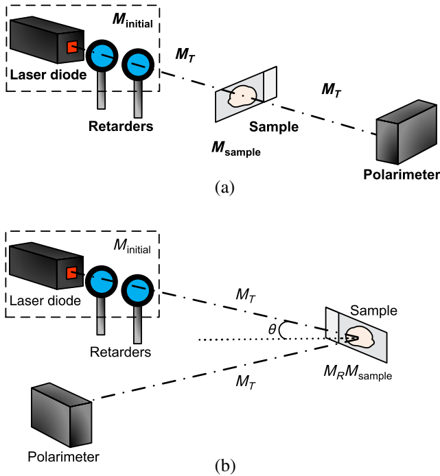
Fig. 7 Transmittance (a) and back-reflection (b) experiment modes. M_T : transmission Mueller matrices, M_R : reflection Mueller matrices, M_{\text{initial}} : Mueller matrices of input light, M_{\text{sample}} : Mueller matrices of sample, \theta : incident angle.
