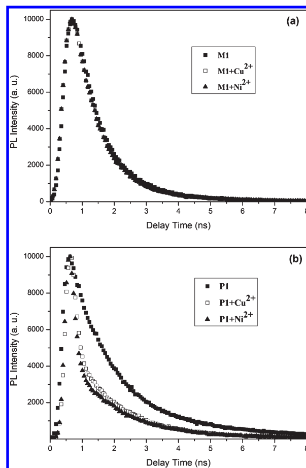
Figure 3. (a) TRF of M1 (solid squares), M1+ Cu^{2+} (open squares) and M1+ Ni^{2+} (solid triangles); (b) TRF of P1 in the absence (solid squares) and in the presence of Cu^{2+} (open squares) and Ni^{2+} (solid triangles) ions. The concentrations of M1 and P1 were 5 \times 10^{-6} M dissolved in THF solutions containing different metal ions ( 2.5 \times 10^{-6} M ).
