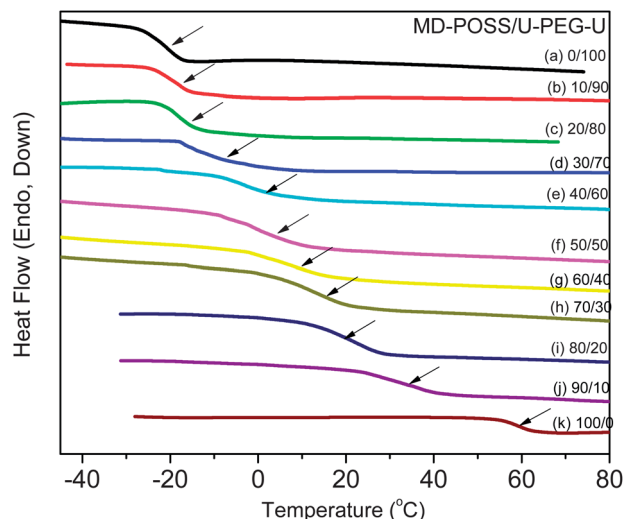
Fig. 6 DSC thermogram of U-PEG-U/MD-POSS blended systems.
