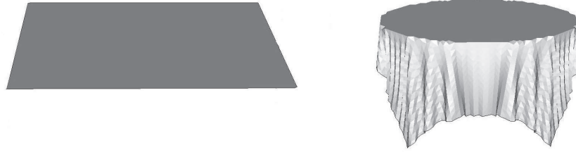
Figure 8: Simulation of a table cloth draping under the gravitational force. The fabric constraint automatically adjusts the parts of the cloth. The spring model of the fabric gives a realistic motion of the cloth. The characteristic eigen frequency for the fabric model in this simulation is \sqrt{k/m} = 1000 and the friction constant is \kappa = 0.1 .
