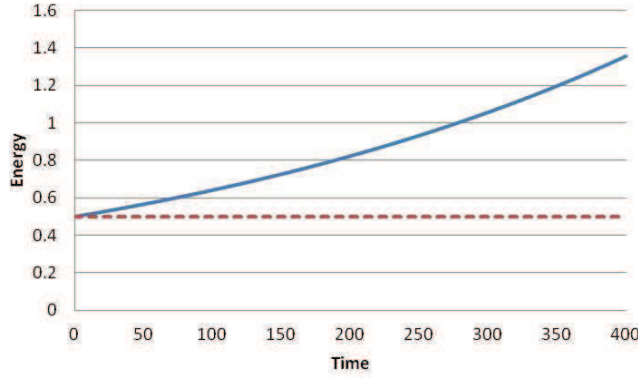
Figure 6: Comparison of the second and fourth order schemes for Eq. (3.19) with \omega\Delta t=0.1 over 40,000 time steps. The plot shows the comparison of the total energy. The numerical results show that the second order predictor-corrector method added 1.7 time of the total energy to the initial value after 40,000 time steps while the fourth order Runge-Kutta method only changed 0.05 percent.
