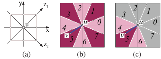
Figure 4: Aligning metro lines with octilinear directions. (a) Octilinear coordinate system around the vertex u , where z_1(u) = (x(u) + y(u))/2 and z_2(u) = (x(u) - y(u))/2 . (b) The corresponding fan-shaped sectors with respect to u . (c) Three sectors to which the optimized version of \overline{uv} belongs.
