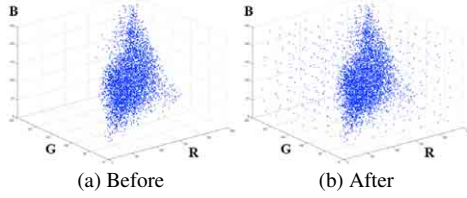
Figure 4: Representative colors in the RGB color space before and after extrapolation.
