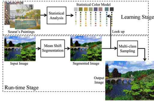
Figure 1: System diagram of our method.
