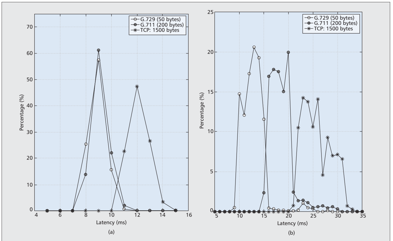
Figure 4. TD-LTE latency histograms for G.729, G.711, TCP transmissions: a) downlink latency histogram; b) uplink latency histogram.
