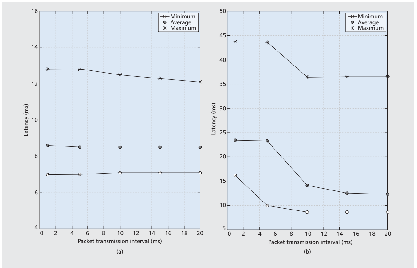
Figure 3. TD-LTE latency vs. packet transmission interval: a) downlink latency; b) uplink latency.
