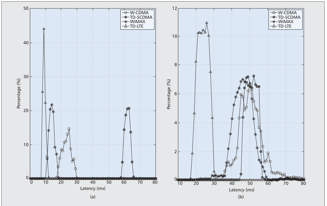
Figure 2. Latency histograms: a) downlink latency histogram; b) uplink latency histogram.
