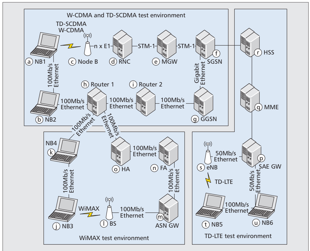
Figure 1. Test environments of W-CDMA, TD-SCDMA, WiMAX, and TD-LTE.
