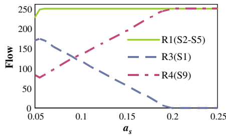
Fig. 5. Influence of maximum violation probabilities on route choice.
