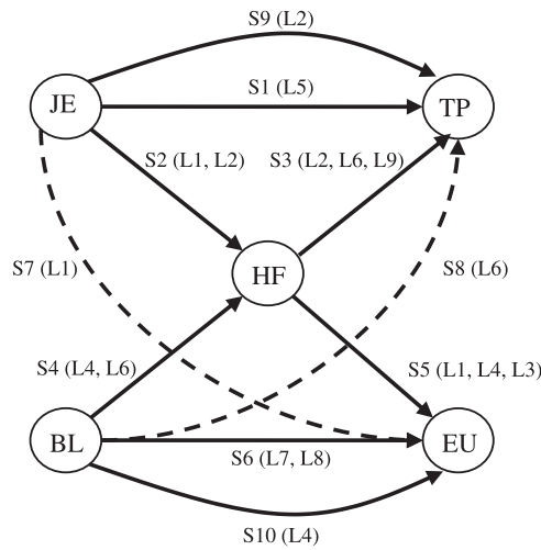
Fig. 2. Transit network representation using links.
