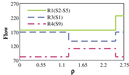
Fig. 7. Influence of the degree of risk aversion of passengers on the flows on R1, R3 and R4.
