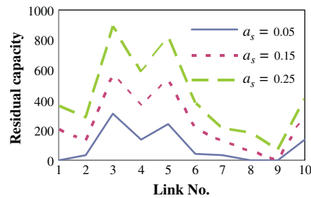
Fig. 4. Residual capacities of links for various \alpha_s values.
