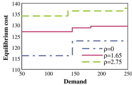
Fig. 6. Influence of the degree of risk aversion of passengers between OD pair 1 on equilibrium cost.
