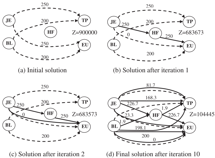
Fig. 8. Illustration of the proposed solution method.
