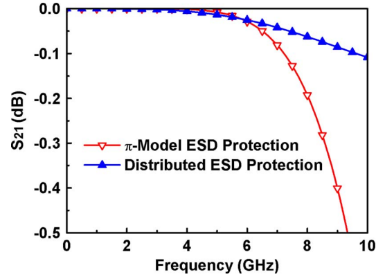
Fig. 24. Simulation results of \pi -model ESD protection scheme and distributed ESD protection scheme with equal-size ESD diodes.
