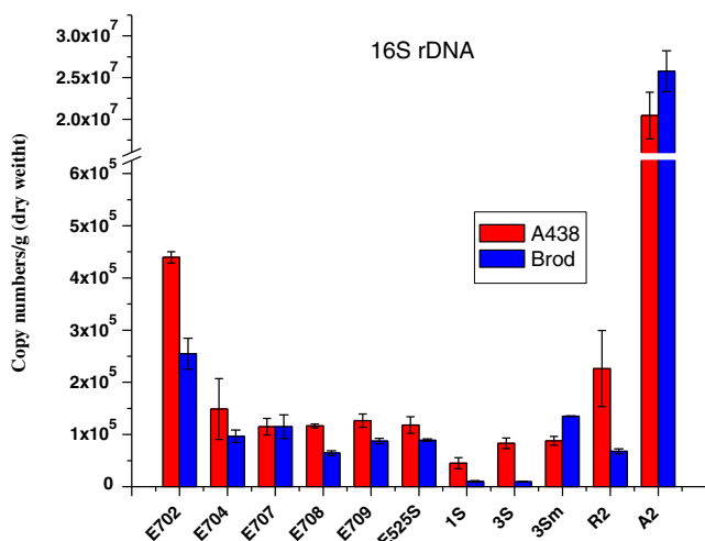
Fig. 3 A comparison of the abundance of anammox bacteria in the 11 samples indicated by abundance of 16S rRNA gene copies with PCR primer set A438 and Brod. Error bars represent standard deviations of triplicate experimental analyses
