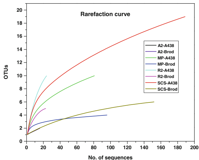
Fig. 1 Rarefaction curves of anammox bacteria 16S rRNA gene PCR-amplified sequences retrieved from different environmental samples with 3 % difference cutoff. MP Mai Po Nature Reserve; SCS South China Sea; R2 freshwater reservoir; A2 wastewater treatment plant. Primer sets used were indicated immediately after the sample name
