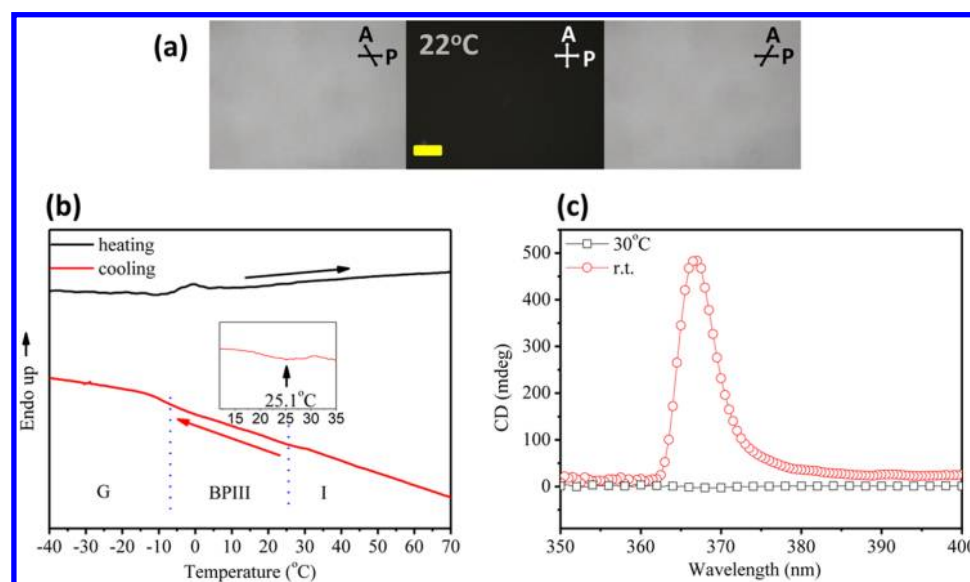
Figure 2. (a) POM images (scale bar = 40 \mu\text{m} ), (b) DSC curves (with rate of 5°C/min upon cooling; inset = isotropic-BPIII transition), and (c) CD signals of OXD7*.
